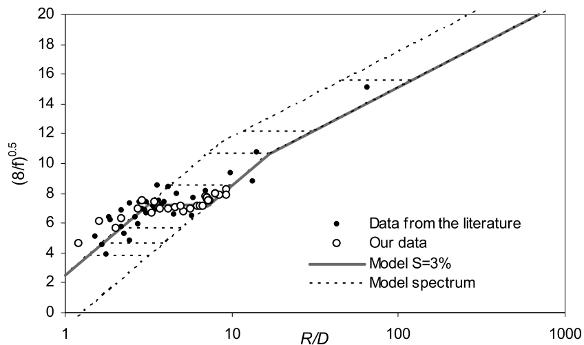
Figure 4. Comparison between data and the flow resistance model (bold line) on slope 3% (horizontal dashed lines represent the model spectrum in domain 2 for slopes 0.1, 0.5, 1, 2, 5, 7, and 9% from top to bottom).
