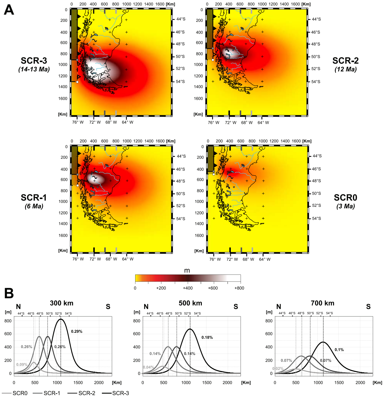
Figure 11. (a) Map of the uplift of the overriding plate resulting from the episodic subduction of 4 ridge segments below South America accompanying the northward migration of the CTJ. White and gray dots mark the position of the CTJ before and after the subduction of each ridge segment, respectively. (b) Topographic profiles parallel to the trench direction at 300 km, 500 km, and 700 km from the trench for each triple junction migration increment. The boundary between regions of northward and southward tilt for each longitudinal profile (dotted lines) shifts toward the north, delineating sectors with different tilt history.
