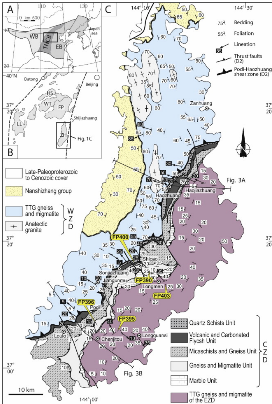
Fig. 1. (A) Simplified map of the North China Craton showing the three-fold subdivision from Zhao et al. (2001). (B) Location of the Zanhuang Massif within the Trans-North China Orogen. LL = Lüliang Massif; HS = Hengshan Massif; WT = Wutaishan Massif; FP = Fuping Massif; ZH = Zanhuang Massif. (C) Proposed structural map of the Zanhuang Massif, with the Western, Central and Eastern Domains described in this study.
