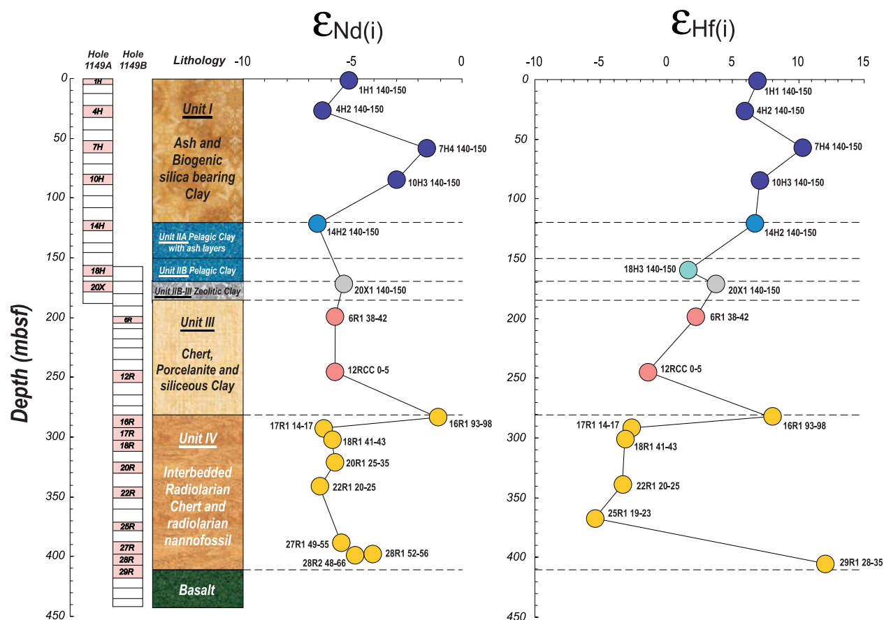
Figure 4. The \epsilon_{\text{Nd}(i)} and \epsilon_{\text{Hf}(i)} values of Site 1149 sediments plotted versus depth in the sedimentary pile.
