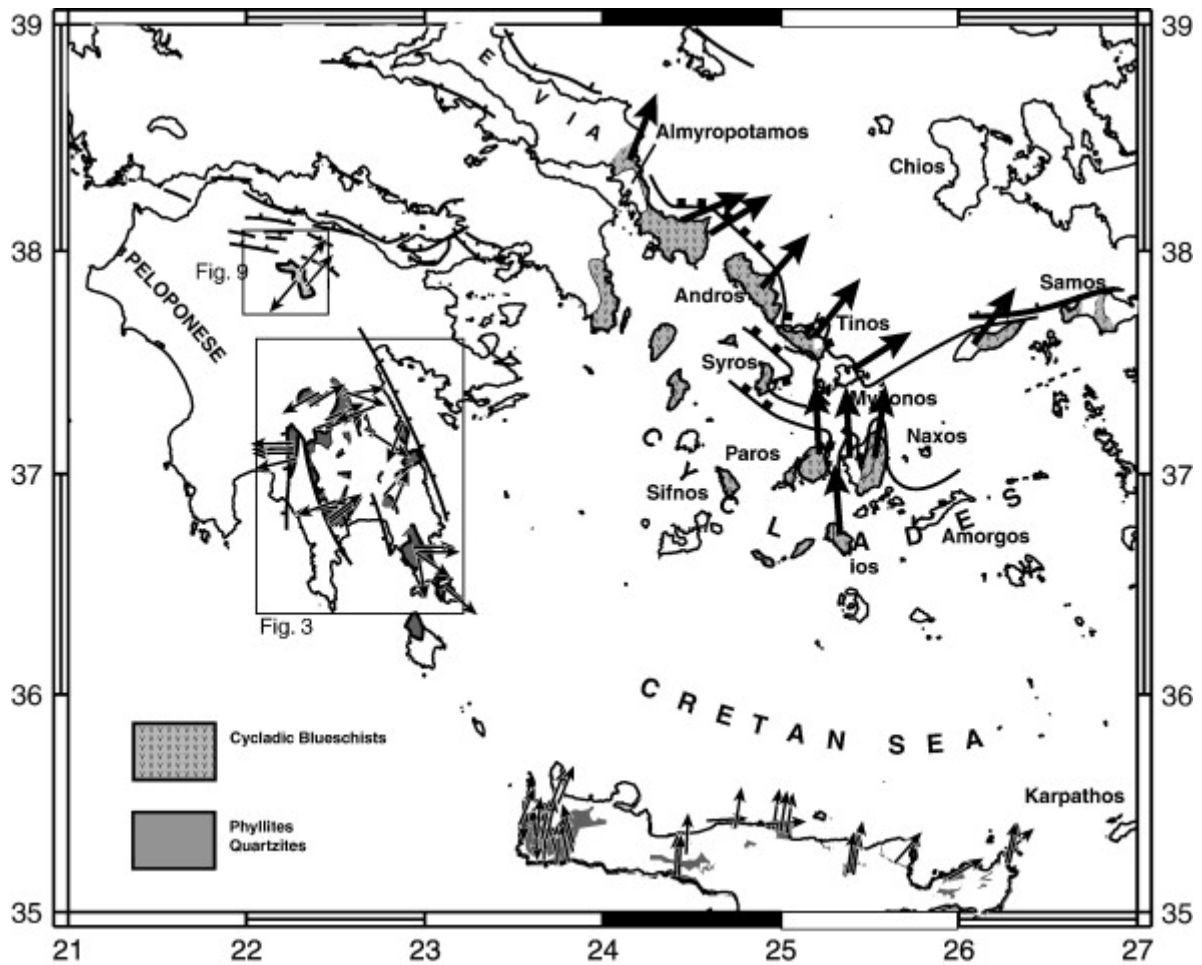
Fig. 2. Map of the Cyclades, Peloponnese and Crete showing the main outcrops of the HP–LT metamorphic rocks. Arrows shows the direction of retrograde stretching lineations of Oligo-Miocene age and the associated kinematic indicators after ([Gautier et al., 1993], [Jolivet et al., 1994a], [Jolivet et al., 1996], [Doutsos et al., 2000], [Trotet, 2000] and [Xypolias and Doutsos, 2000]). Large arrows for the Cyclades, smaller arrows for the PQ Nappe.
