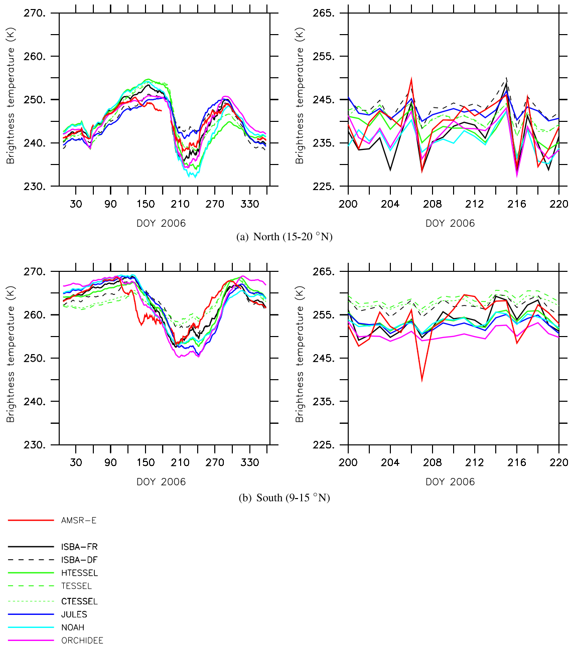
Figure 4. Temporal evolution (time in DOY) of simulated and observed horizontally polarized brightness temperature (K) from the eight ALMIP-MEM simulations (CMEM configuration 10 of Table 1). Brightness temperatures are spatially averaged for the (a) north and (b) south of the studied window. (left) Annual cycle with a running average of 15 days. (right) Variability on shorter temporal scale is depicted between DOY 200 and 220. For each LSMs, a bias correction was applied on the basis of the mean annual mean bias computed on each subwindow.
