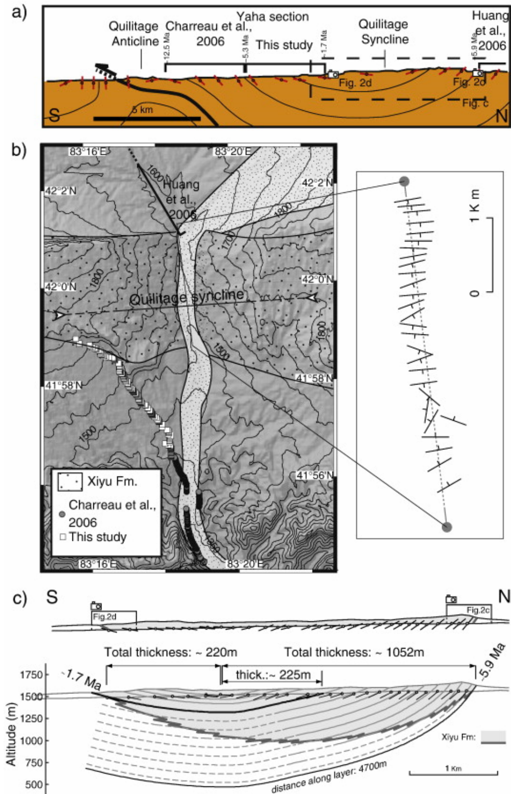
Fig. 4. (a) Simplified cross section of the Quilitage anticline and syncline with the locations of the different magnetotstratigraphic studies which provide bound on the basal ages of the Xiyu Formation; (b) Topographic map of the Yaha river with location of the magnetotstratigraphic sampling sites of Charreau et al. (2006) and this study; (c) Detailed balanced cross section of the Quilitage syncline with location of the 29 structural measurements and the exact position of the two lithological transitions between the Xiyu conglomerates and underlying Neogene Kuche Formation.
