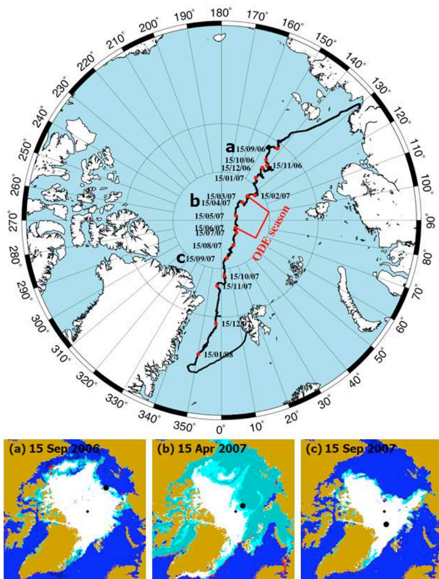
Fig. 1. Track of the TARA drift (September 2006–January 2008). Top panel: TARA drift track across the Arctic Ocean with the time period of ODE season marked in red and locations a, b, and c corresponding to the time of the three QuikSCAT sea ice maps below. Bottom panels: QuikSCAT sea ice maps for 15 September 2006 (a), 15 April 2007 (b), and 15 September 2007 (c). The colors are brown for land, blue for open water, cyan for first year ice, turquoise for mixed ice, and white for multi-year ice. In each map, the small black dot marks the North Pole and the large black dot represents the TARA location. Note that TARA was near the multi-year ice edge on 15 September 2006, and TARA was also located near the multi-year ice edge, which had migrated close to the North Pole by 15 April 2007, indicating the rapid advection of the multi-year ice pack along the Transpolar Drift Stream. This rapid evacuation of multi-year sea ice toward the West Arctic left a vast region in the East Arctic for first-year sea ice to form behind TARA.
