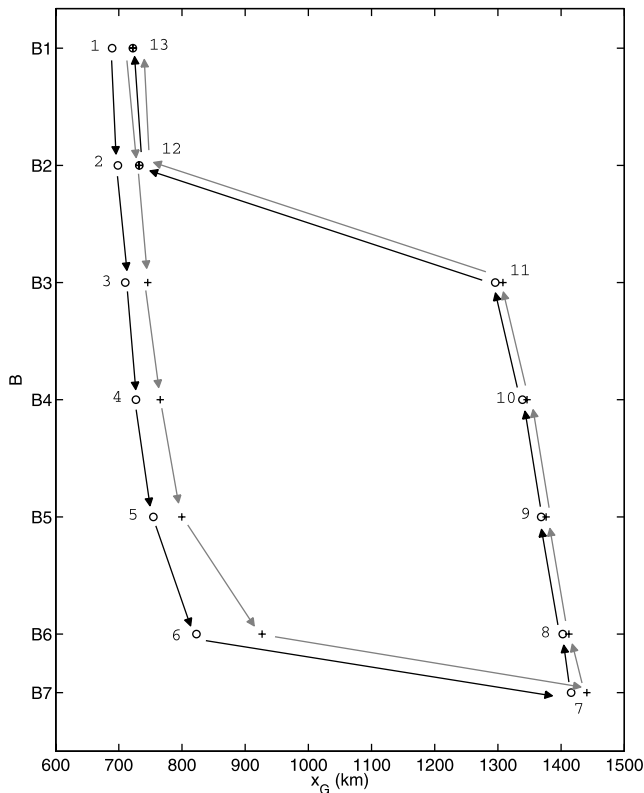
Figure 5. Evolution of the steady grounding line position versus the applied fluidity (open circles) for step 1 to step 13 of simulation HYST. Crosses depict results obtained by BL theory (Schoof, personal communication, 2008).
