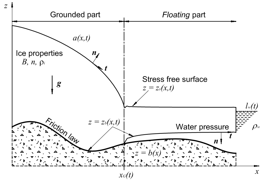
Figure 1. Geometry and nomenclature of the investigated problem.
