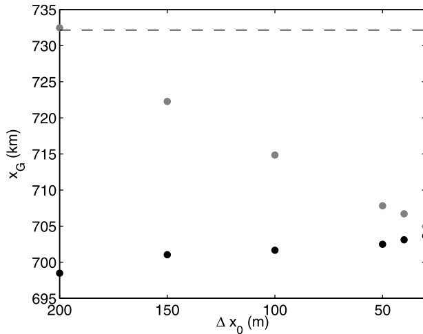
Figure 6. Evolution of the steady grounding line position as a function of the horizontal mesh extension \Delta x_0 . Black circles (gray circles) represent results obtained for simulations starting from the steady state obtained after HYST step 2 (HYST step 12). Dashed line depicts results obtained by BL theory (Schoof, personal communication, 2008).
