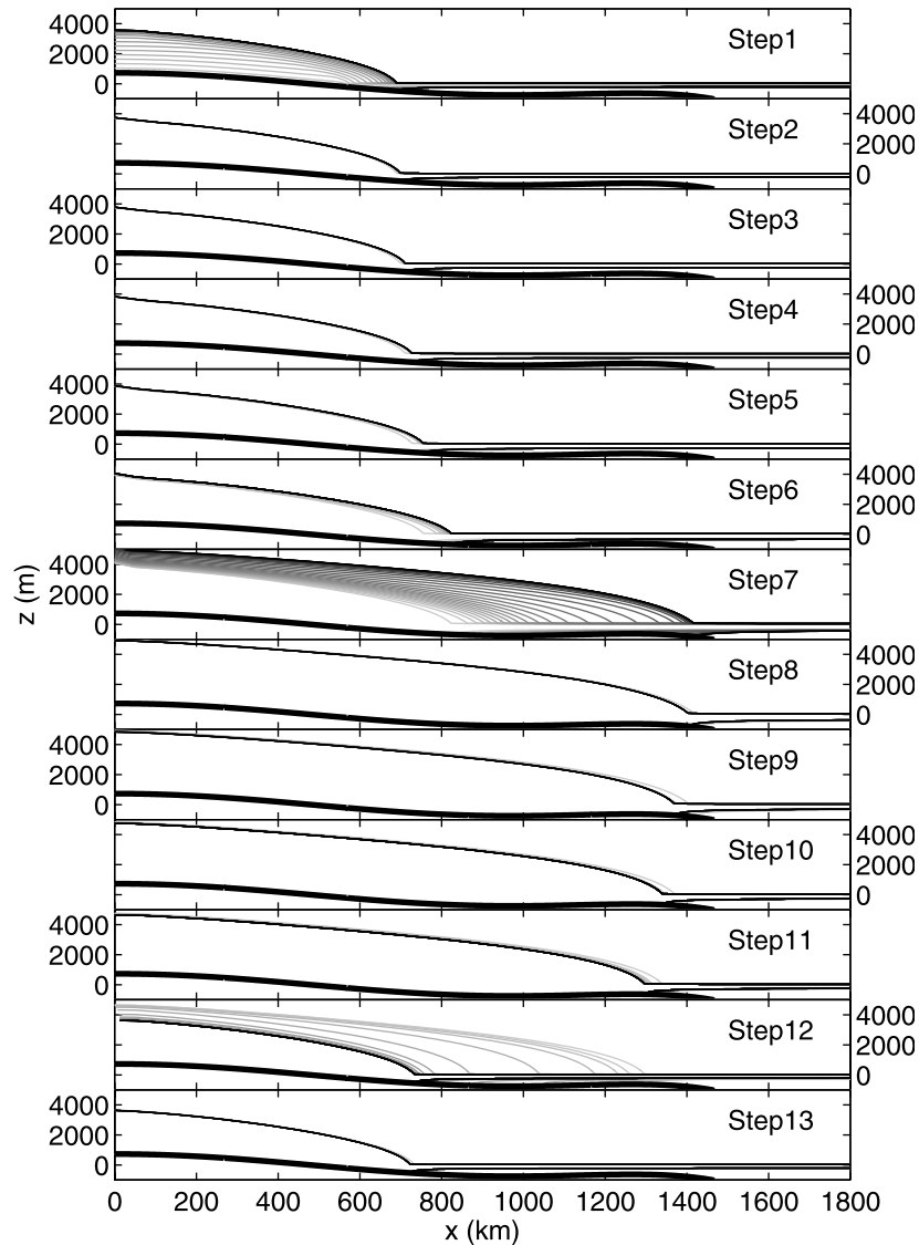
Figure 4. Surface profiles obtained every 1000 years in gray level for step 1 to step 13 of simulation HYST. The steady state profile for each step is plotted with a black line. Duration and prescribed fluidity for each step are defined in Table 2.
