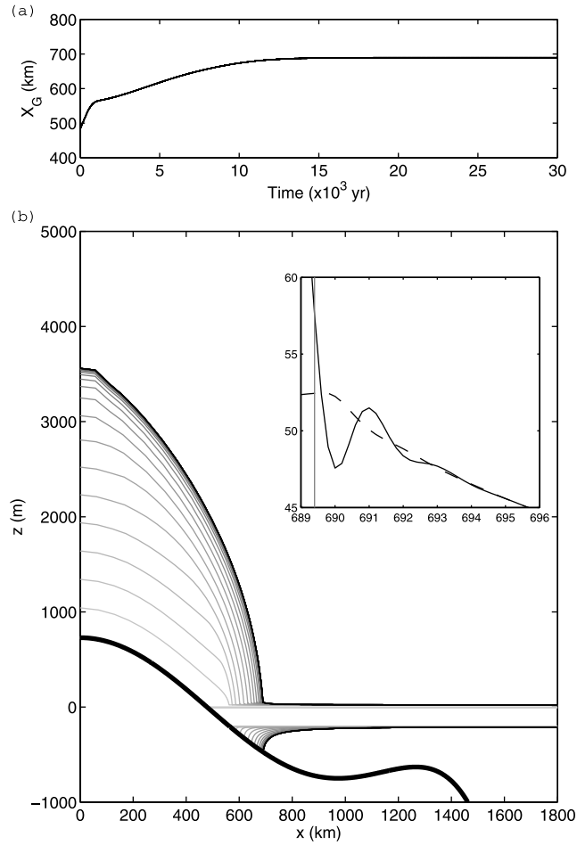
Figure 2. (a) Evolution of x_G over time for the first step of simulation HYST. (b) Surface profiles plotted every 1000 years. The steady state surface is plotted in black. The inset shows an enlargement of the upper surface (solid line) and is compared to the profile obtained for the floating surface (dashed line), whereas the vertical gray line marks the position of x_G .
