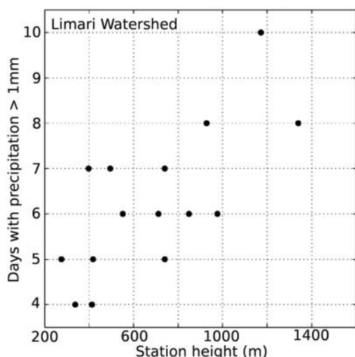
Figure 12. Variation of precipitation frequency with station altitude for sites in the Limari catchment for the period 1 May–30 September 2006.
