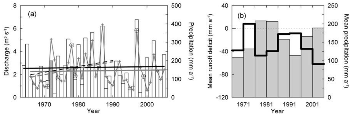
Figure 4. Historical variation of precipitation and discharge at the high-elevation La Laguna Embalse station (P15 and R10 in Figure 1, 30^{\circ}12'S , 70^{\circ}03'W , 3130 m asl). (a) Open bars are annual precipitation, and solid gray lines are annual discharge. Missing precipitation and discharge data that were replaced by measurements downstream at the Varillar station (P23 and R14 in Figure 1, 29^{\circ}56'S , 70^{\circ}32'W , 860 m asl) are indicated by gray bars and open circles, respectively. Continuous and dashed black lines are precipitation trends over the periods 1964–2005 and 1966–1990, respectively. Continuous and dashed gray lines are discharge trends over the periods 1964–2005 and 1966–1990, respectively. Runoff and precipitation increasing trends over the period 1964–1990 only have a low level of significance ( p = 0.06 ), and no significant trend is observed for the period 1964–2005. (b) Variation of 5-year mean precipitation and runoff deficit at La Laguna Embalse station between 1966 and 2005. Gray columns are mean precipitation, and black line is mean runoff deficit.
