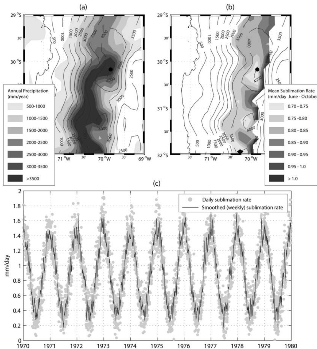
Figure 8. (a) Annual mean precipitation (rain + snow) simulated by WRF for the period 1970–1980. Black contour lines represent the model topography and coastline. (b) Mean daily sublimation rate during winter and spring (June–October, inclusive) at model grid points where snow is present at least 90% of the time. (c) Time series of daily sublimation rates (gray circles) at the point indicated by the black circle in Figures 8a and 8b. The solid line shows the sublimation after applying a 7-day smoothing filter.
