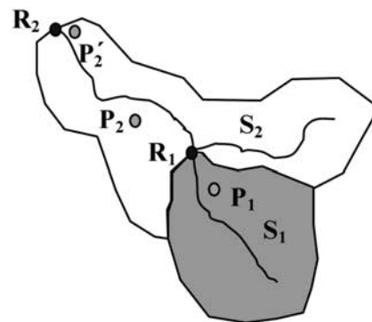
Figure 5. Example of the methodology used to estimate catchment scale precipitation for runoff coefficient calculations.
