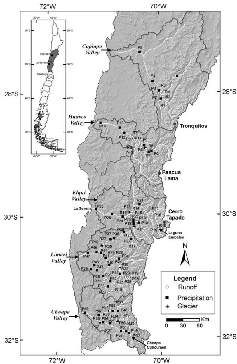
Figure 1. Map of Norte Chico region showing the runoff stations (white points), rain gauges (black squares), and main glaciers (gray circles). Names and characteristics of the stations are defined in Tables 1 and 2.
