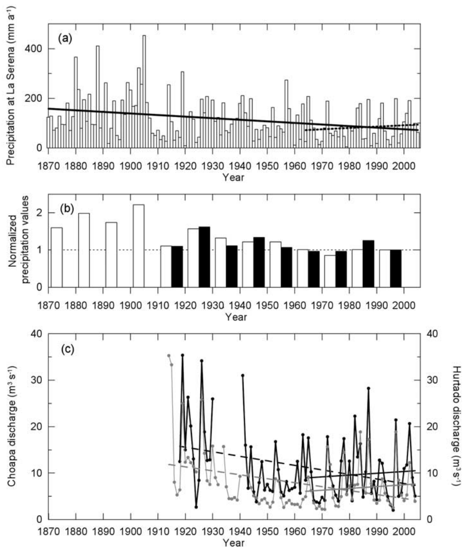
Figure 3. Historical variation of precipitation and discharge. (a) Annual precipitation at La Serena (P25 in Figure 1, 142 m asl) between 1870 and 2005. Continuous and dashed lines are linear regressions for the periods 1870–2005 and 1964–2005, respectively. Precipitation decrease at La Serena between 1870 and 2005 is significant ( p = 0.001 ), whereas no significant trend was observed after 1964. (b) Normalized decadal precipitation at La Serena (open bars) and Puerto Oscuro (black bars, P59 in Figure 1). Data are normalized by dividing decadal precipitation by the mean precipitation during the decade 1991–2000. (c) Annual discharge between 1918 and 2005. Dotted black line is discharge of Choapa River at Cuncumen data (R32 in Figure 1, 1200 m asl), and dotted gray line is discharge of Turbio River at Varillar (R14 in Figure 1, 860 m asl). Continuous and dashed lines are linear regressions for the periods 1918–2005 and 1950–2005, respectively. The runoff decrease of Turbio River and Choapa River between 1918 and 2005 is significant ( p = 0.006 ), whereas the observed increase after 1950 is not statistically significant.
