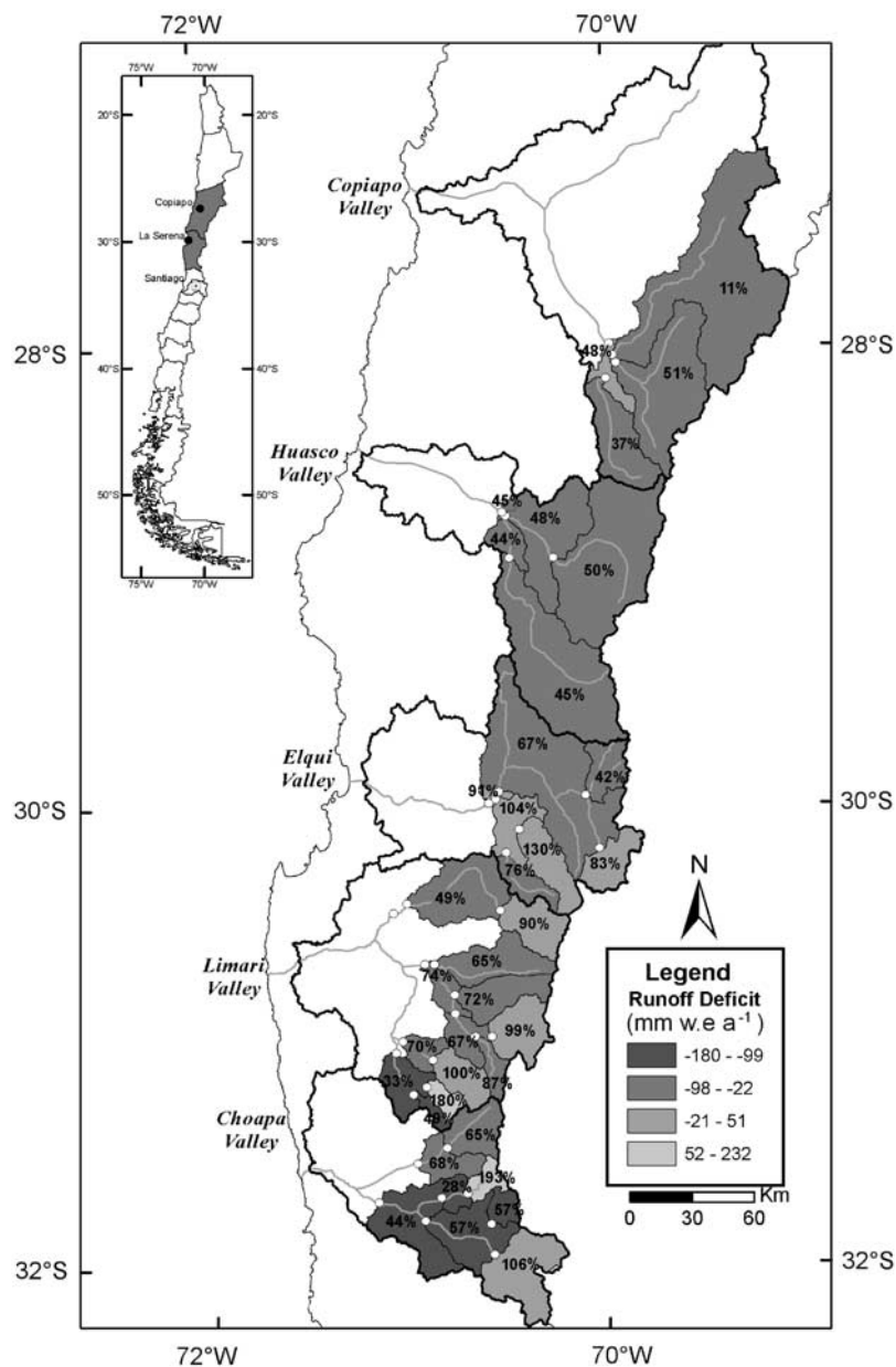
Figure 6. Runoff coefficients and runoff deficit values (in \text{mm w.e. a}^{-1} ) for catchments in the Norte Chico region.
