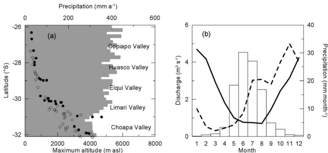
Figure 2. (a) Evolution of precipitation with latitude. Open circles are annual mean precipitation at sites lower than 750 m asl; filled circles reflect precipitation at sites higher than 750 m asl. Gray horizontal bars indicate the maximum altitude of the Andes at 0.16° intervals. (b) Seasonal variation of precipitation and discharge in Norte Chico region. The open bars are mean monthly precipitation between 1900 and 2005 at La Serena-La Florida airport (P25 in Figure 1, 29°54'S, 71°12'W, 142 m asl). The continuous line is mean monthly discharge at La Laguna Embalse station (R10 in Figure 1, 30°12'S, 70°02'W, 3130 m asl) between 1964 and 2005. The dashed line is monthly discharge of Hurtado River at Recoleta Dam (R30, 30°28'S, 71°04'W, 410 m asl) between 1928 and 1984.
