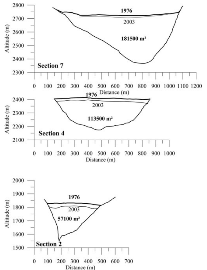
Fig. 2. Cross-sections 7 (a), 4 (b) and 2 (c). The horizontal and vertical scales are the same for all cross-sections. The surface area values correspond to the year 1976. The cross-sections are seen from the downstream.
