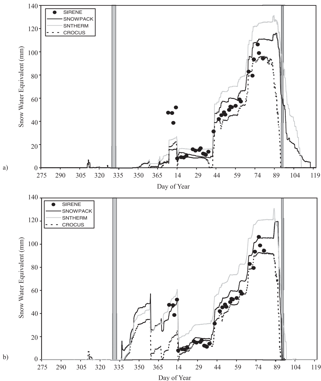
FIG. 4. SWE simulations from SNOWPACK, CROCUS, and SNTHERM using (a) SIRENE and (b) NARR meteorological information for the 2004/05 winter. Gray bars represent the duration between the first snow accumulation and melting observations from the Sherbrooke-A and Lennoxville Environment Canada weather stations.
