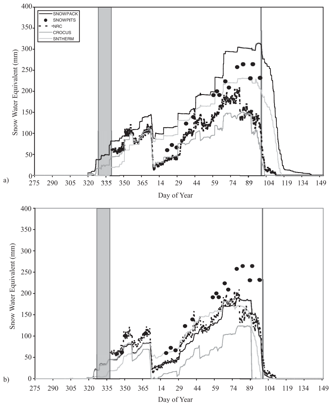
FIG. 6. Same as Fig. 4, but for the 2007/08 winter.
