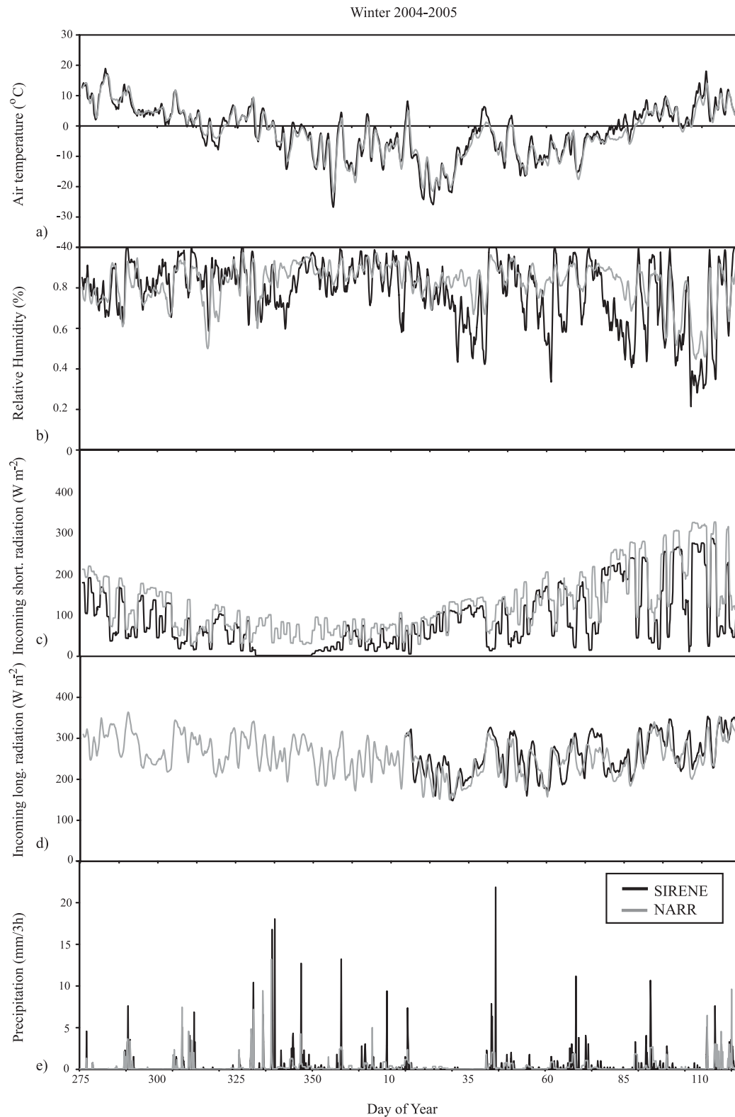
FIG. 2. Temporal evolution of (a) air temperature, (b) RH, (c) incoming shortwave radiation, (d) incoming longwave radiation, and (e) precipitation measured at the SIRENE station and from NARR data during the 2004/05 winter season.
