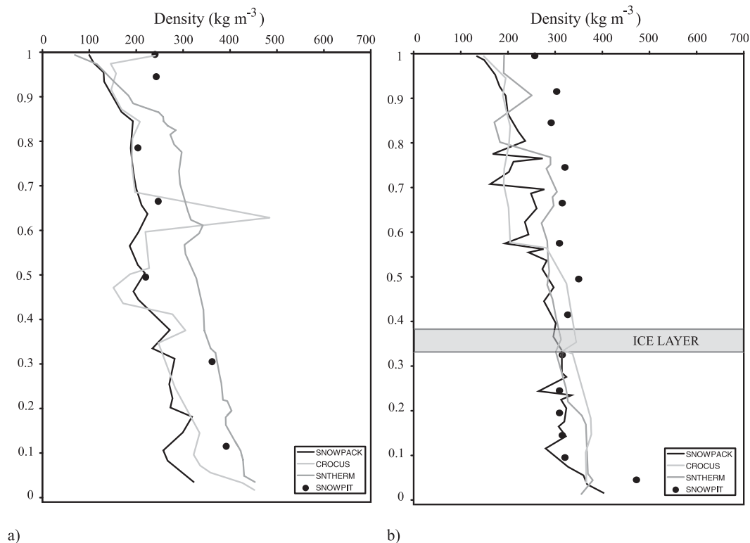
FIG. 7. Modeled and measured vertical profile comparison of density for (a) day 76 of 2005 and (b) day 70 of 2008.
