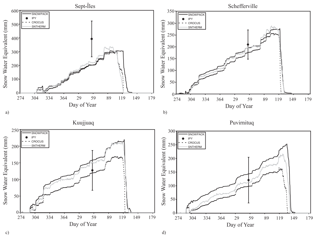
FIG. 8. Comparison between predicted and measured SWE values at (a) Sept-Îles, (b) Schefferville, (c) Kuujuaq, and (d) Puvirnituk using SNOWPACK during the IPY project.
