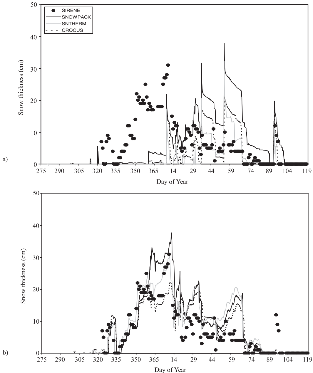
FIG. 5. Snow thickness simulations from SNOWPACK, CROCUS, and SNTHERM using (a) SIRENE and (b) NARR meteorological information for the 2005/06 winter.
