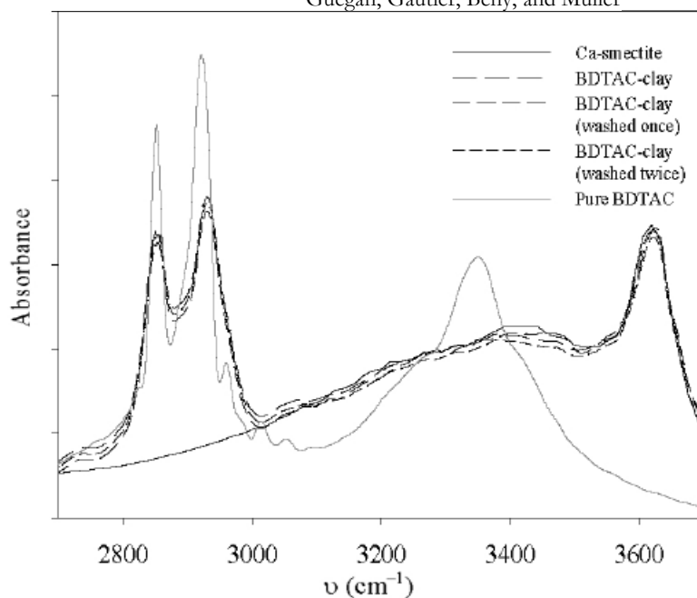
Figure 2. FTIR spectra of pure BDTAC, BDTAC-clay, BDTAC-clay (washed once), and BDTAC-clay (washed twice) at the concentration of 1.31 \times 10^{-2} \text{ mol L}^{-1} (i.e. 4 x CEC) and Ca-smectite, over the wavenumber range 2700–3700 \text{cm}^{-1} .
