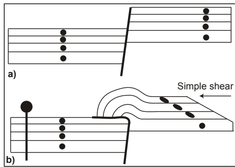
Fig. 4 An attempt to integrate the concept of "fault-fold" in a balanced cross-section. To balance the structure (same as step b on Fig. 2), layers have to be subject to a simple shear which characteristics depend on the inherited fault net slip.
