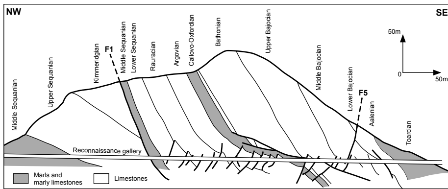
Fig. 7 Geological cross-section of the "Bois du Peu" tunnel. Same label for faults as in Fig. ??. Modified after CETU (1999).
