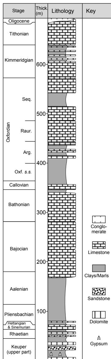
Fig. 3 Synthetic lithologic log of the Besançon area showing the alternation of clays/marls soft levels with hard limestone layers. The main décollement level is located within the upper Keuper layers; Pliensbachian-Aalenian, Oxfordian-Argovian and middle Sequanian layers may serve as secondary décollement levels. Oxf. s.s. : Oxfordian sensu stricto . Arg.: Argovian. Raur.: Rauracian. Seq.: Sequanian.
