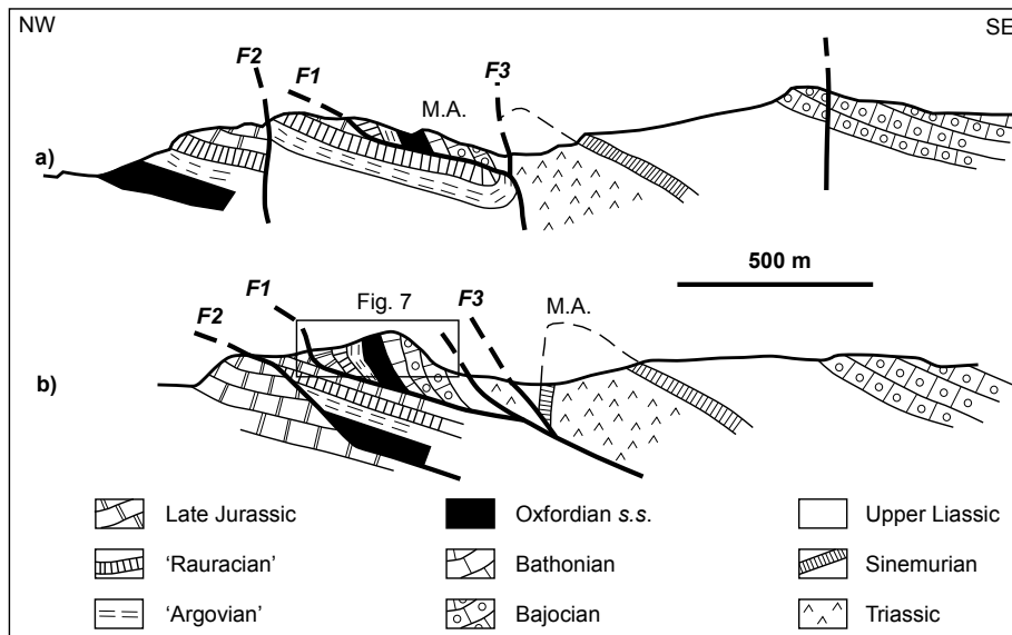
Fig. 8 Cross-sections of the "Bois du Peu" area. a: Interpretation in term of "fault-fold" (after Glangeaud, 1951; Chauve and Perriaux, 1974). Same label for faults as in Fig. ???. The fault associated to the "fault-fold" structure corresponds to F1 and to the lower part of F3. The upper part of F3 would be the result of a late reactivation (Dreyfuss in Chauve, 1975, p. 54). b: Proposed interpretation according to new data and balanced cross-sections. See text for details.
