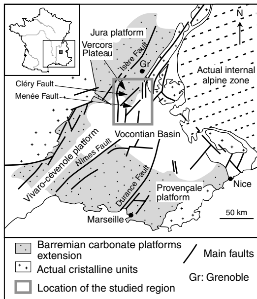
FIG. 1. — Palaeogeographic map of the Vocontian Basin and surrounding carbonate platforms during the Barremian times. Adapted from Jacquin et al. (1991).
