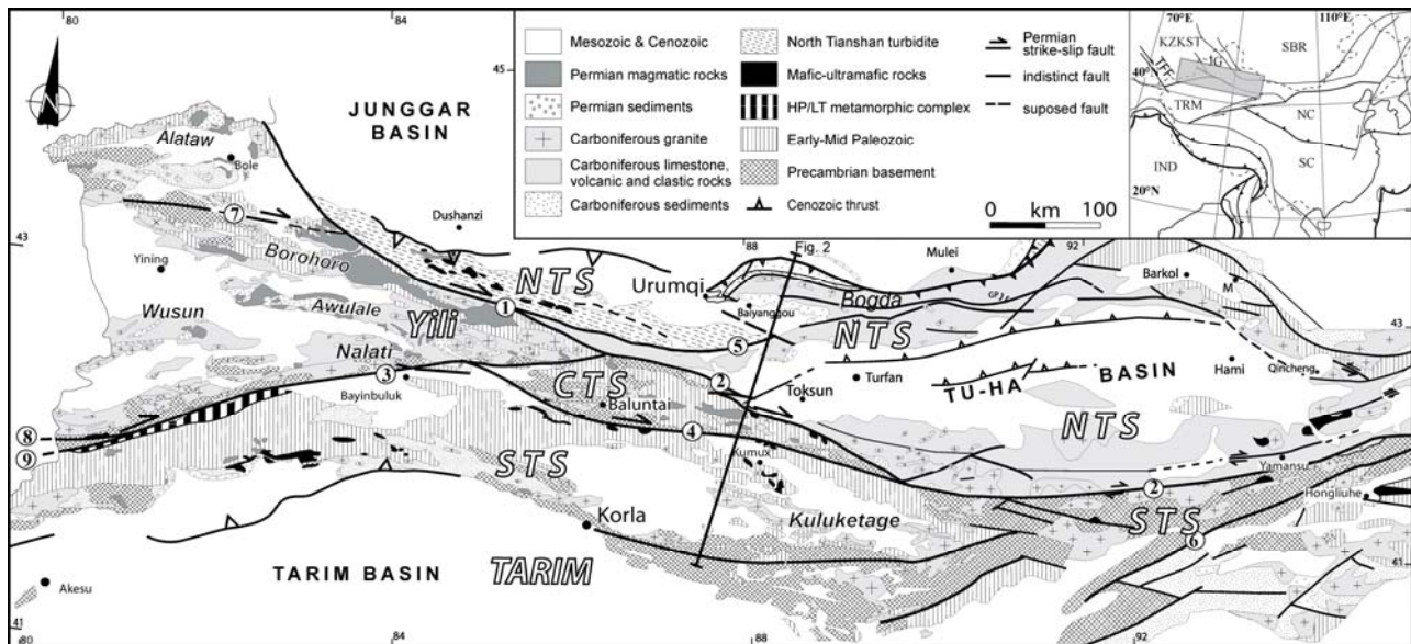
Figure 1 : Geological and structural map of Chinese Tianshan. Location of cross-section of figure 2.
