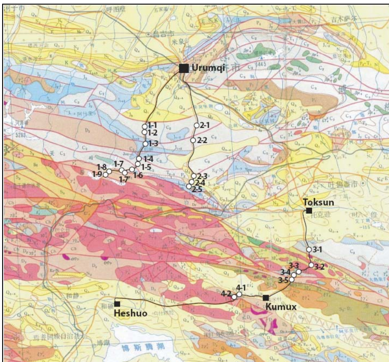
Fig. 4. Geological map and the circuit for Days 1 to 4 .
