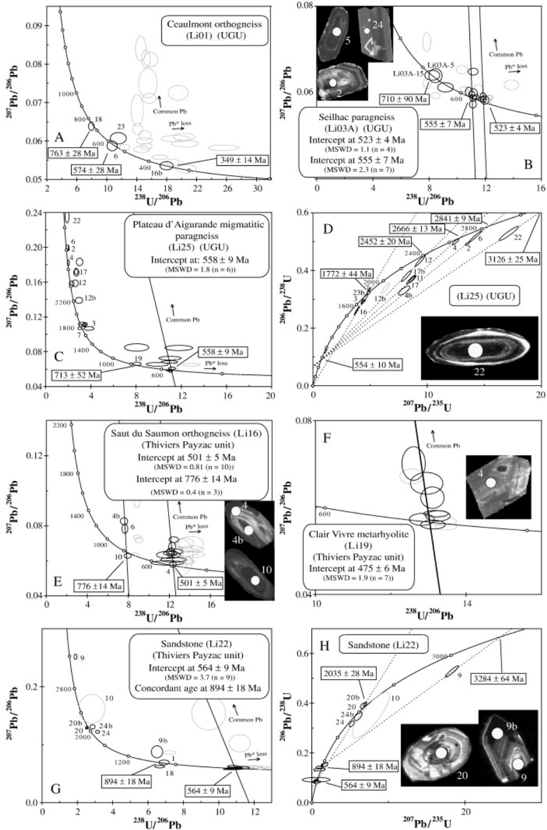
Fig. 6. Inverse (A, B, E, F, G) and normal (D, H) concordia diagrams reporting zircon U–Pb data in samples of the Upper Gneiss Unit and Thiviers–Payzac Unit. Examples of CL images of zircon are shown with location of analytical points. The diameter of ablation pit is ca. 20 \mu m. Data-point error ellipses are plotted as 2\sigma .
