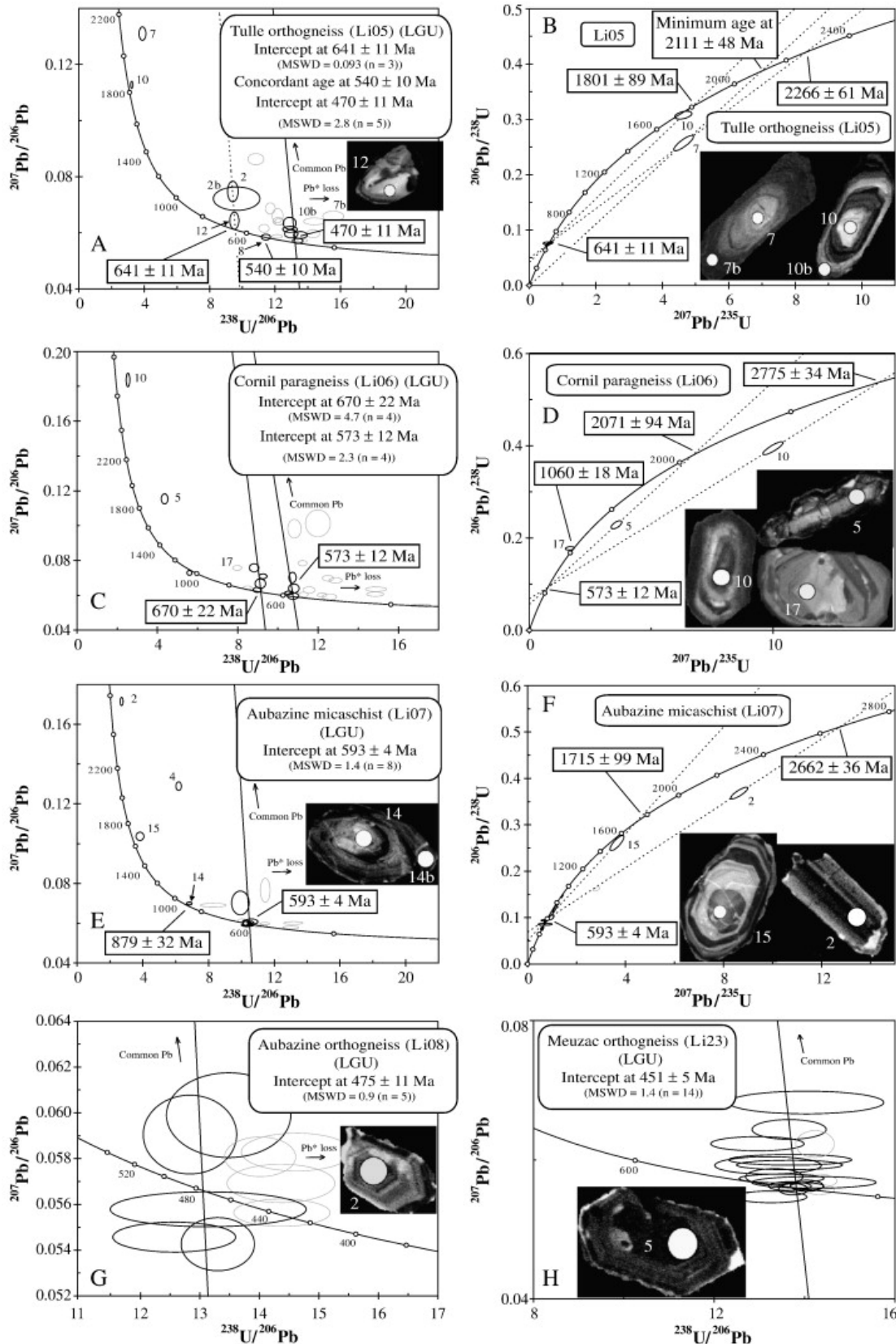
Fig. 4. Inverse (A, C, E, G, H) and normal (B, D, F) concordia diagrams reporting zircon U–Pb data in samples of the Lower Gneiss Unit. Examples of CL images of zircon are shown with location of analytical points. The diameter of ablation pit is ca. 20 \mu\text{m} . Data-point error ellipses are plotted as 2\sigma .
