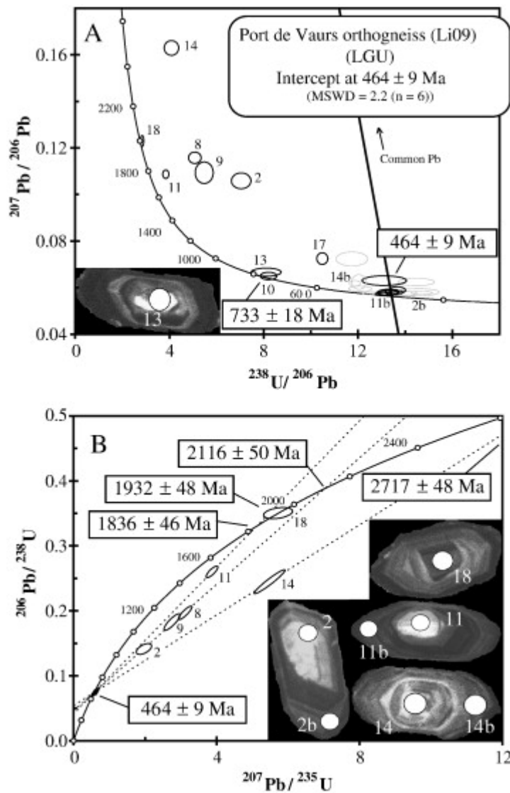
Fig. 5. Inverse (A) and normal (B) concordia diagrams reporting zircon U–Pb data in samples of the Lower Gneiss Unit. Examples of CL images of zircon are shown with location of analytical points. The diameter of ablation pit is ca. 20 \mu\text{m} . Data-point error ellipses are plotted as 2\sigma .
