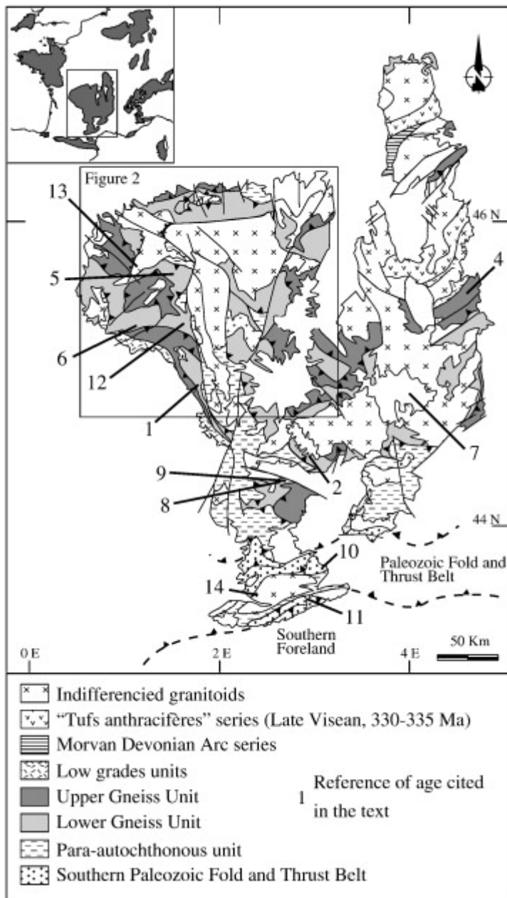
Fig. 1. General geological map of the French Massif Central with localizations of ages cited in the text (modified after Faure et al., 2005).
