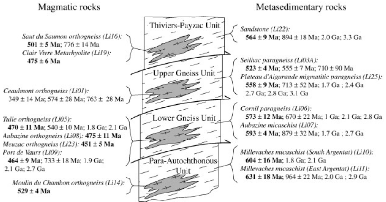
Fig. 7. Schematic diagram summarizing the various U–Pb on zircon ages obtained in the different tectonostratigraphic units of the Limousin area. Bold ages are indicating the maximum deposition ages for the metasedimentary formations and magmatic emplacement ages for the orthogneiss
