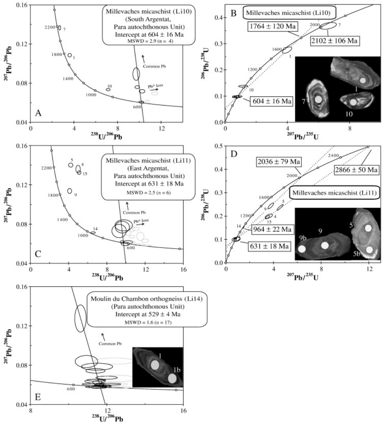
Fig. 3. Inverse (A, C, E) and normal (B, D) concordia diagrams reporting zircon U–Pb data in samples of the Para-Autochthonous Unit. Examples of CL images of zircon are shown with location of analytical points. The diameter of ablation pit is ca. 20 \mu m. Data-point error ellipses are plotted as 2\sigma .
