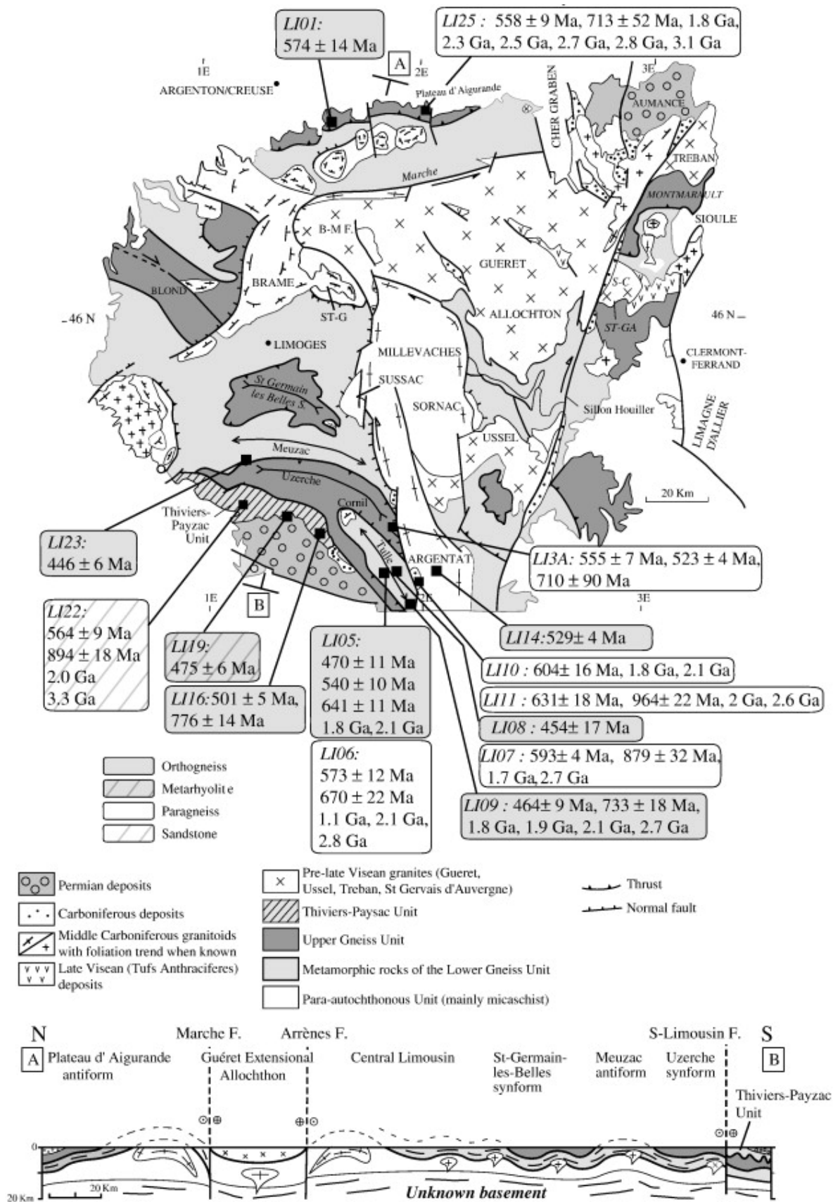
Fig. 2. Geological sketch map and N-S cross section of the Limousin area, and samples localizations.
