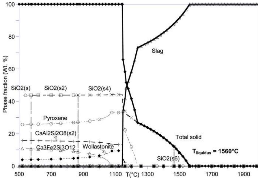
Figure 3. Weight percent of the phases formed as a function of the temperature for C1 without Na 2 O and K 2 O.
