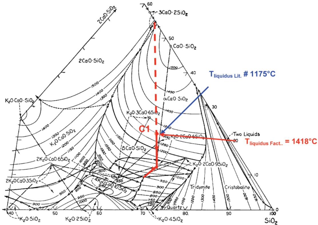
Figure 2. Ternary diagram \text{SiO}_2\text{--CaO--K}_2\text{O} [13].
