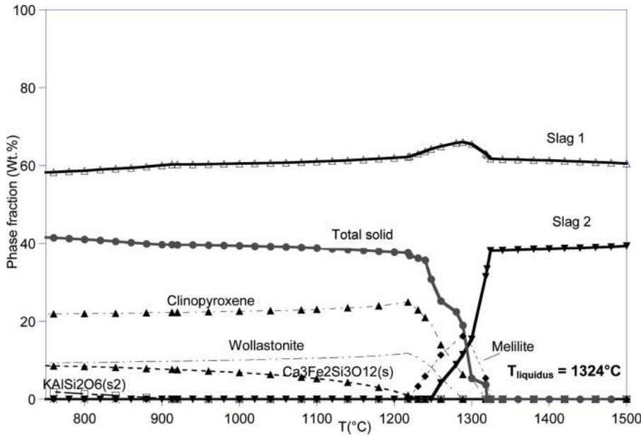
Figure 4. Weight percent of the phases formed as a function of the temperature for C1 with Na 2 O and K 2 O.
