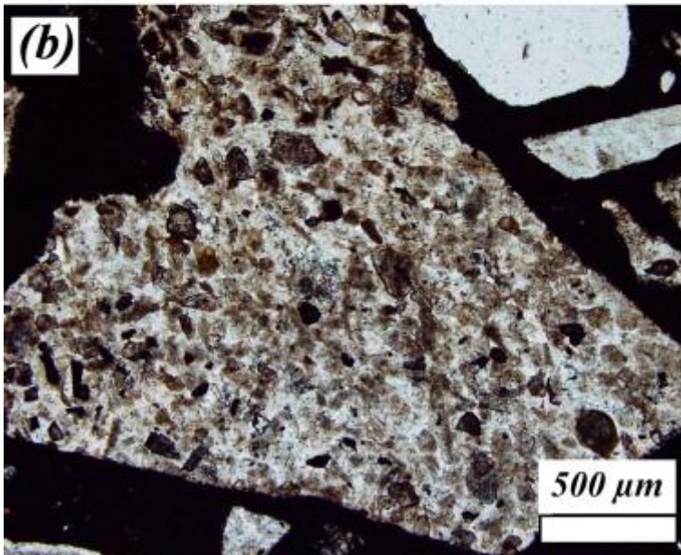
Fig. 8. Optical view of the volcanic protoliths (a) in the middle of the section (distance from the exposed surface 4 mm) with a dark appearance and (b) at the back of the sample (distance from the exposed surface 8 mm).
