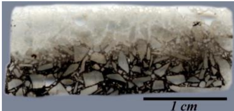
Fig. 5. Polished thin section 30 \mu\text{m} thick of the Kitty's Gap Chert sample after atmospheric re-entry. The fusion crust is at the top, denoted by a thin (<1 mm) bright white layer. Note the dark colour of the cement in the lower part of the image.
