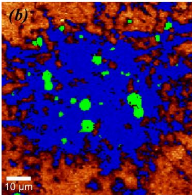
Fig. 9. Optical and Raman images of a melted hydromuscovite grain located at 1.9 mm from the exposed surface. The H 2 O-filled bubbles are clearly highlighted by Raman spectroscopy (colour coding: brown for quartz, blue for melted hydromuscovite and green for water). (For interpretation of the references to colour in this figure legend, the reader is referred to the web version of this article.)
