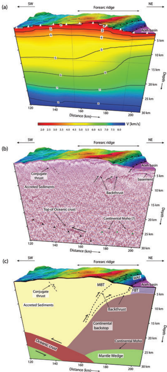
Figure 5. (a) 3-D block diagram showing the P -wave velocity model obtained by first arrival traveltimes tomography along the black line on Fig. 1, and seafloor bathymetry. All distances marked are from the subduction front. Contours are marked for every 1 \text{ km s}^{-1} . The water depth varies from \sim 2700 \text{ m} in the Aceh basin (purple) to \sim 255 \text{ m} on forearc ridge (red). White triangles are the positions of OBSs within the length (87.5 km) of the profile shown. (b) 3-D block diagram of depth converted seismic reflection image of Fig. 2b. Locations of backthrusts, conjugate fault, reflections from top of the oceanic crust and continental Moho have been marked. Black and green triangle pointers have been marked to highlight reflections from the top of downgoing oceanic crust and the continental Moho, respectively. (c) Schematic diagram of interpreted tectonic features at the forearc high of the north Sumatra Margin. Continental backstop and Moho are determined from the interpretation of the seismic reflection and refraction results.
