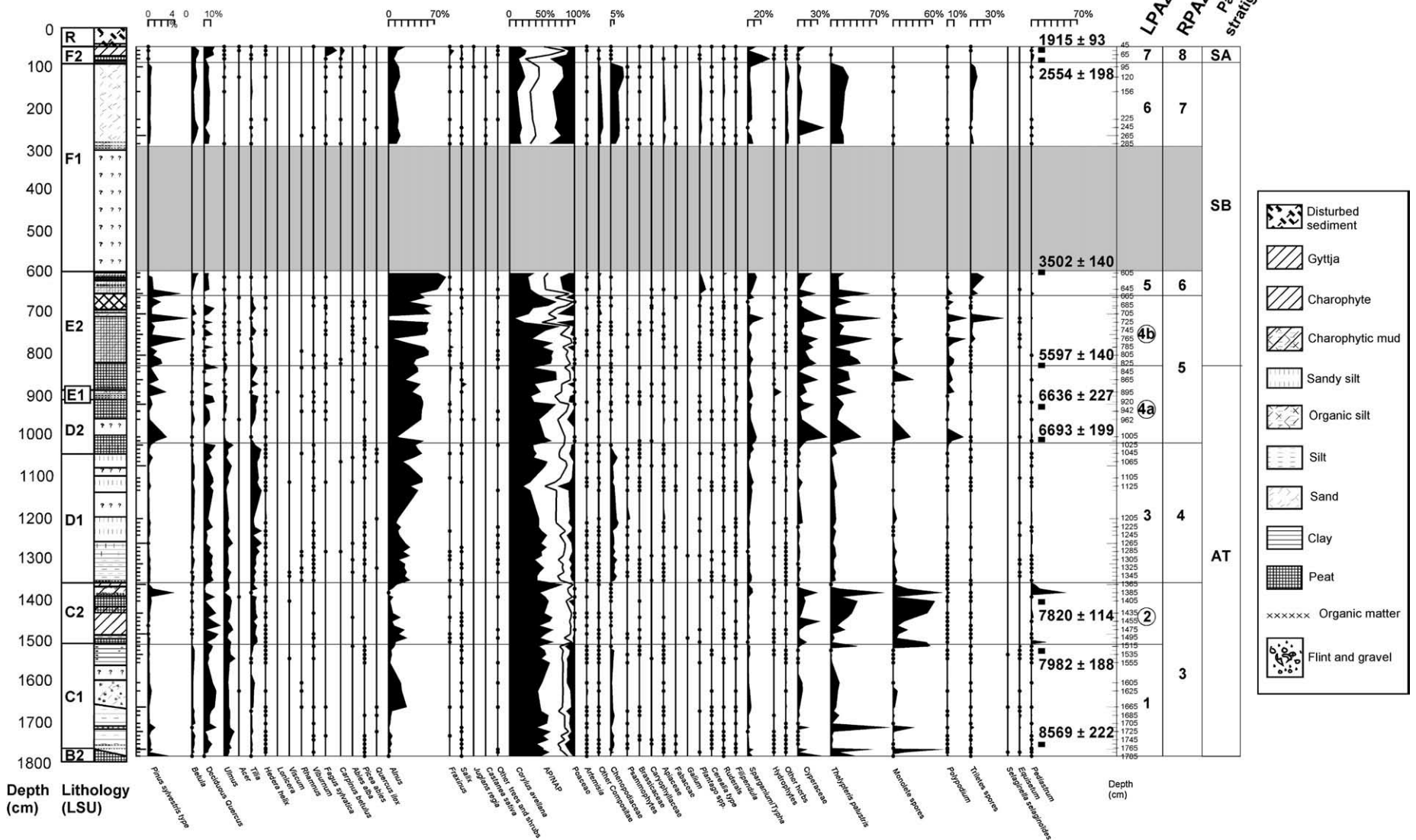
Fig. 4. Pollen diagram (simplified) from borehole S2 at St-Momelin. Radiocarbon dates are (2σ) calibrated years BP (Before Present). RPAZ: Regional Pollen Assemblage Zone; LPAZ: Local Pollen Assemblage Zone; LSU: LithoStratigraphic Units. Distorted zones due to high Thelypteris pollen concentration are indicated by black circles in the LPAZ column. Shaded area: sediment lost during coring or non fossiliferous sediment. AT: Atlantic; SB: Subboreal; SA: Subatlantic.
