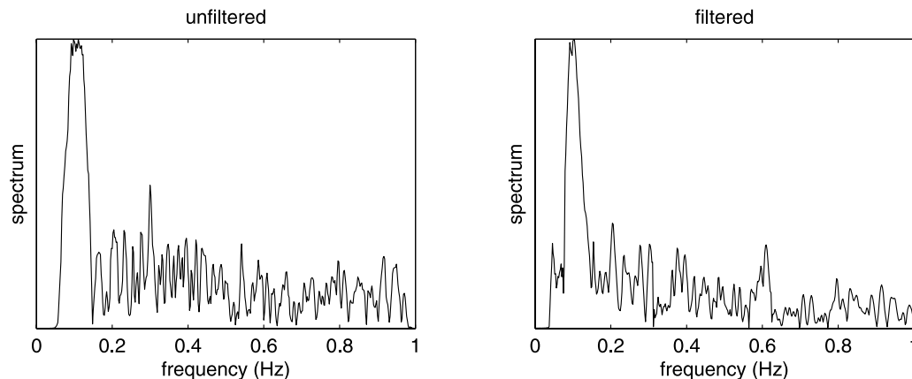
Figure 7. A comparison of the spectra of the total stack of the data plotted in Figures 5 and 6, respectively. Although there are small differences, we note that their general similarity would indicate that the improvement in the signal-to-noise ratio is not at the expense of bandwidth.
