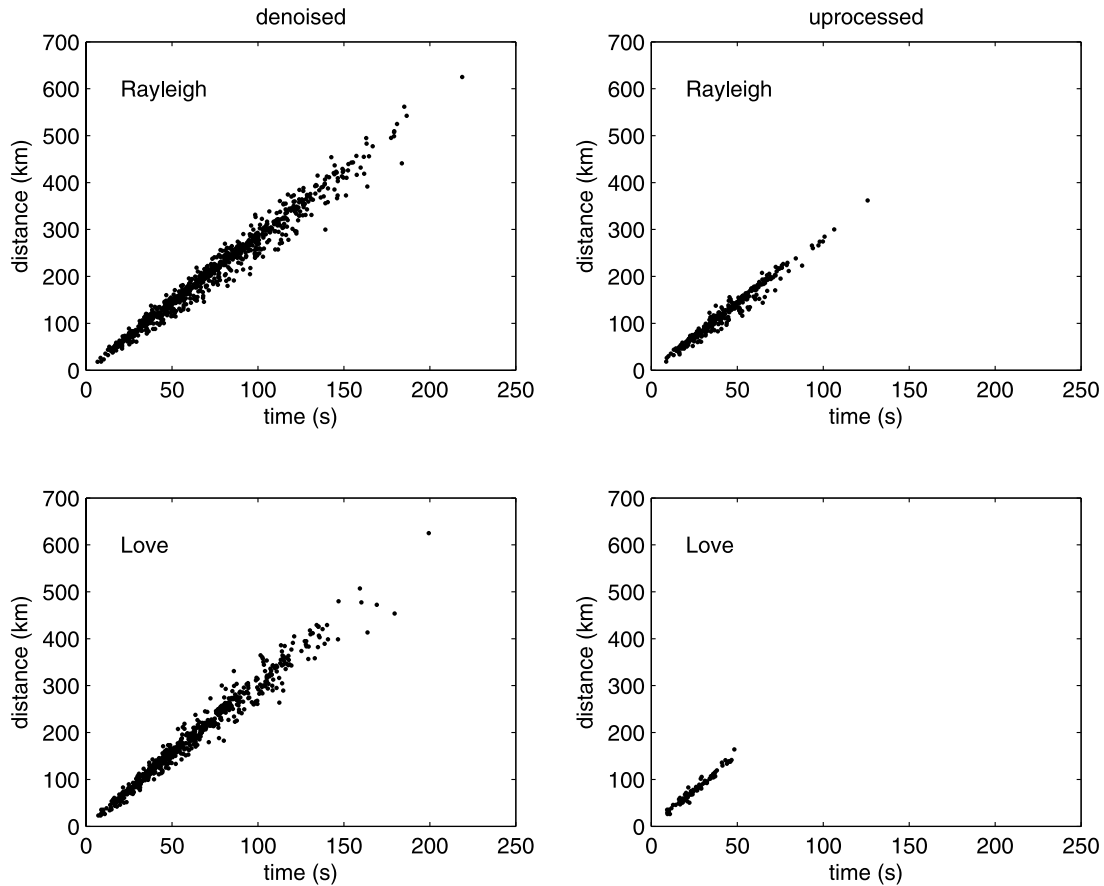
Figure 8. Measured 8s surface wave traveltimes versus distance plots. (top left) Denoised Rayleigh wave traveltimes. (top right) Unprocessed Rayleigh wave traveltimes. (bottom left) Denoised Love wave traveltimes. (bottom right) Unprocessed Love wave traveltimes.
