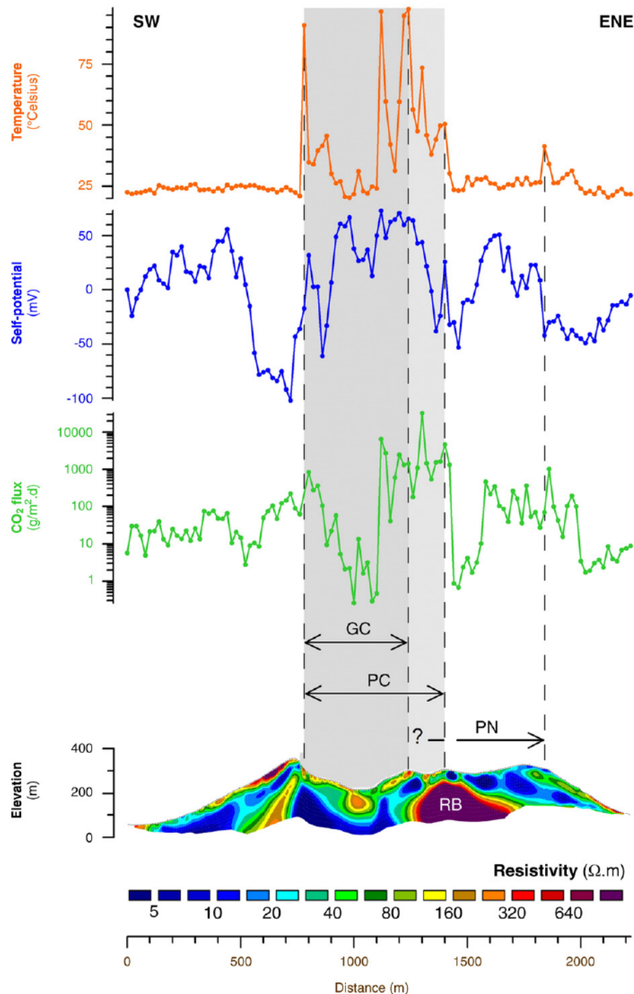
Fig. 8. Temperature, self-potential, soil CO 2 flux, and electric resistivity tomography along Profile 8. Note the presence of a large resistive body under the Punta Nere former cone (see also Profile 1 on Fig. 4). PN: Punta Nere crater, PC: Pietre Cotte crater, GC: Gran Cratere crater.
