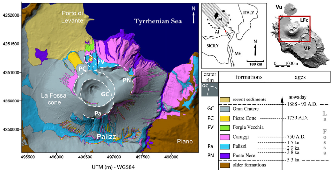
Fig. 1. Location of the studied area. Simplified geological map of La Fossa cone draped on the DEM (map simplified from de Astis et al., 2007 ) and chronology. PN (Punte Nere), Pa (Palizzi), FV (Forgia Vecchia), PC (Pietre Cotte), and GC (Gran Cratere) crater rims are represented. In the upper right corner, Vu, VP, and LFc stand for Vulcanello, Vulcano Primordiale and La Fossa cone. On the location and structural sketch map of the Aeolian Islands area M, AI, TL, and ME stand for the Marsili Oceanic Basin, the Aeolian Islands represented by white ellipses (red star for Vulcano; black shapes for seamounts), the Tindari-Letojanni fault system, and the Malta Escarpment fault system (sketch simplified from Ventura et al., 1999 ).
