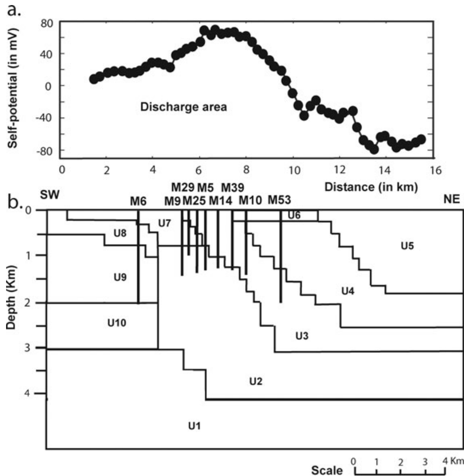
Figure 11. Self-potential data and simplified geological model used for the inversion. The model comprises 10 geological units labelled U1 to U10. (a) The self-potential data are taken from Fitterman & Corwin (1982). (b) The hydrogeological model is taken from the resistivity profile EE' discussed by Wilt & Goldstein (1981). The value of the resistivity of the geological units are taken from Wilt & Goldstein (1981) (their fig. 3) and are reported in Table 2. The self-potential anomaly points out that the flow occurs mainly in Units U2 and U3 (see Corwin et al. 1979).
