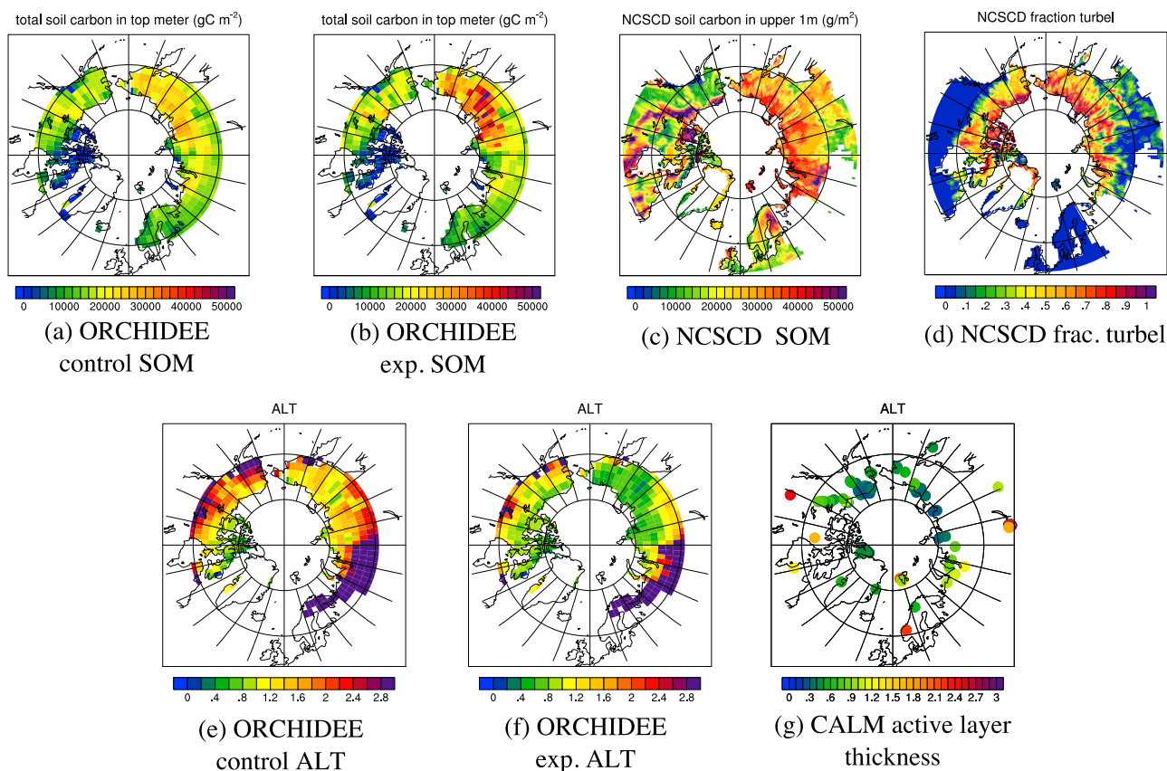
Figure 2. (a) ORCHIDEE soil carbon stocks in top meter, without considering the insulation effect of SOM. (b) ORCHIDEE, with consideration of cryoturbation and insulation effect of SOM. (c) NCSCD Total carbon stocks in top meter of soil. (d) NCSCD fraction of soils in the turbel suborder (cryoturbated, permafrost-affected mineral soils). Active Layer Thickness [m]: (e) ORCHIDEE, without insulation by organic matter, (f) ORCHIDEE with insulation by organic matter, (g) observations from CALM [Brown et al. , 2000].
