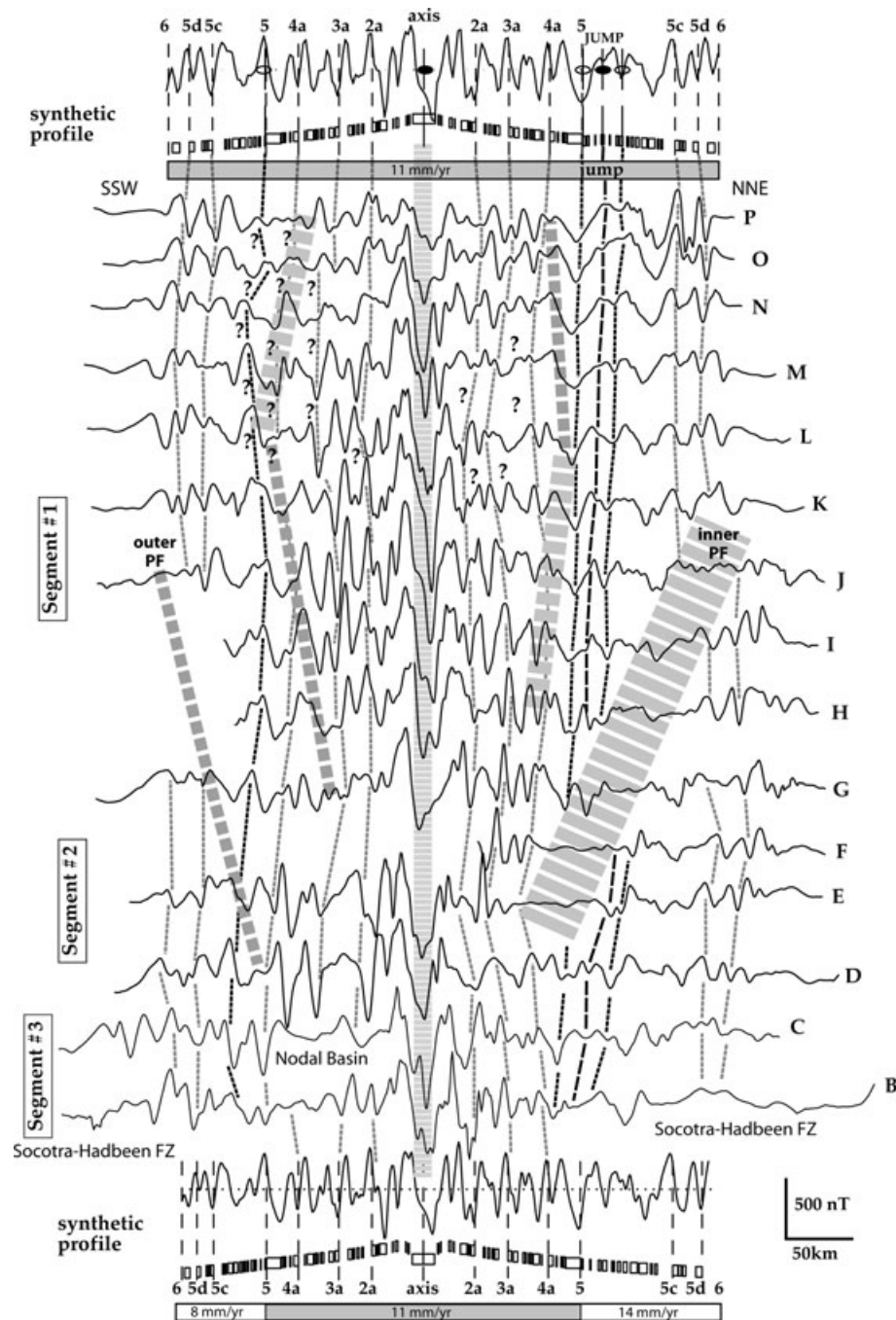
Figure 3. Identification of magnetic anomalies on profiles B to P. Profiles are projected onto the N206°E direction. Top: synthetic profile including ridge jump at 11 Ma, 30 km southward, calculated for constant half spreading rate of 11 mm yr -1 . The black circles indicate the present-day and former ridge axes. The white and black circles correspond to the ridge jump. Bottom: synthetic profiles with asymmetric half spreading rates before 11 Ma. Grey zones correspond to the pseudo-faults: PF. Question marks indicate uncertain pickings.
