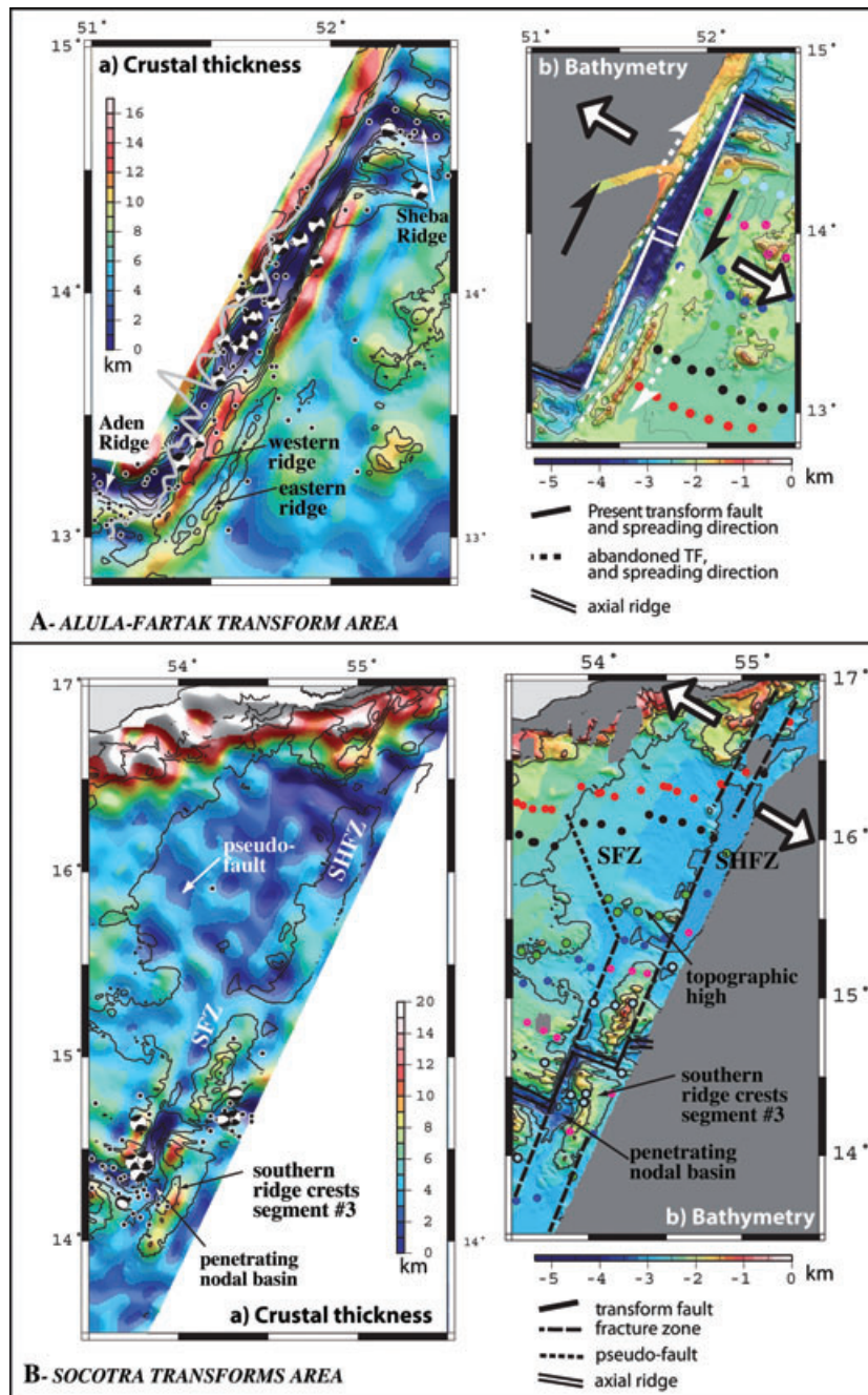
Figure 7. (A) Alula-Fartak Transform Fault: (a) crustal thickness map, with superimposed bathymetric contours (contour interval 500 m). Magnetic profile S is plotted along the ship's track as a grey line. The shallow seismicity is plotted since 1973 (focal depth <50 km; magnitude >2; USGS/NEIC and Harvard database; CMT Focal mechanisms represented on PDE location). (b) Cartoon based on bathymetric map illustrating the counter-clockwise change in spreading direction, which produces extension along the AFTF. A distensive component (open arrows) is already present at the onset of spreading direction change. A new spreading direction occurs immediately after the onset of plate motion change (continuous arrows). Flexural transverse ridges are formed subsequent to the opening episode and the abandonment of transform fault traces. (B) The Socotra and Socotra-Hadbeen Transforms and fracture zones: (a) crustal thickness map, with superimposed bathymetric contours (contour interval 500 m). The shallow seismicity is plotted since 1973 (focal depth <50 km; magnitude >2; USGS/NEIC and Harvard database; CMT Focal mechanisms represented on PDE location). (b) Cartoon based on bathymetric map illustrating the development of segmentation on the two transform faults. See Fig. 5 for legend concerning magnetic anomalies.
