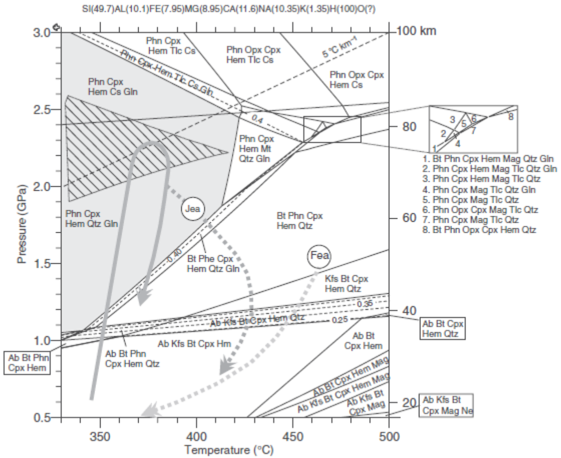
Fig. 9. Isochemical P–T phase diagram showing the stability fields for mineral assemblages in omphacite-rich veins, sample COR-4, using Theriak–Domino. Contours for jadeite content of clinopyroxene are shown as stippled lines. See text for discussion.
