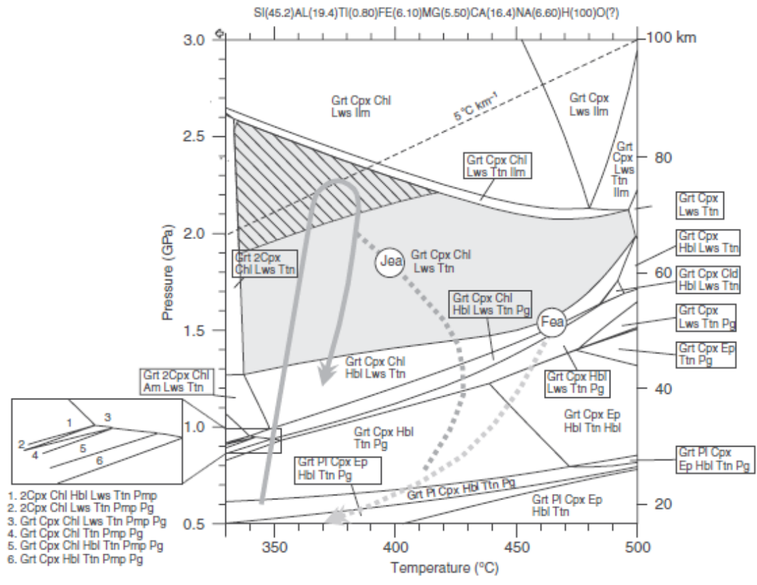
Fig. 8. Isochemical P–T phase diagram showing the stability fields for mineral assemblages in sample COR-4 matrix, calculated using Theriak–Domino. See text for discussion. Note that at 0.9–2.6 GPa and <340 °C two coexisting clinopyroxenes can be stable.
