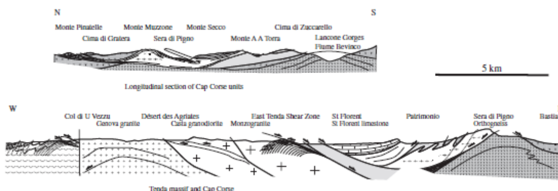
Fig. 2. N-S (a) and E-W (b) cross-sections of northern Corsica (modified from Jolivet et al., 1998) showing the main tectonic units and the locations of blueschist to eclogite facies pseudotachylytes and the eclogite facies rocks in the area. Notice that the De'file' du Lanco' ne lawsonite eclogite locality is positioned at a low structural level.
