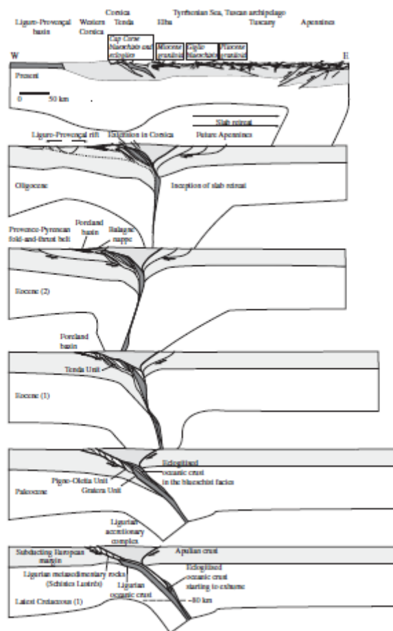
Fig. 10. Model of tectonic evolution of the Alpine LHP metamorphic complexes Corsica (modified from Jolivet et al., 1998), where the new P–T data from lawsonite eclogites in De'file' du Lanco' ne have been incorporated. See text for discussion and details.
