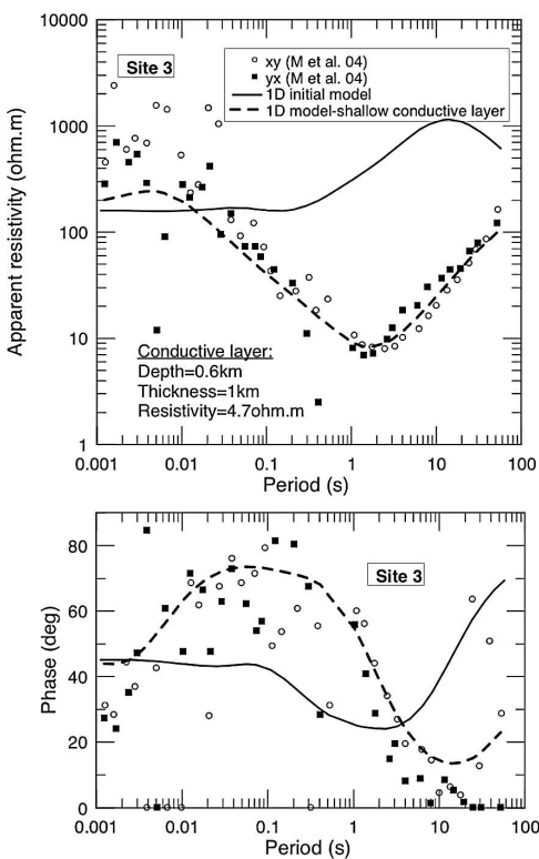
B) Superficial conductor - best fit
