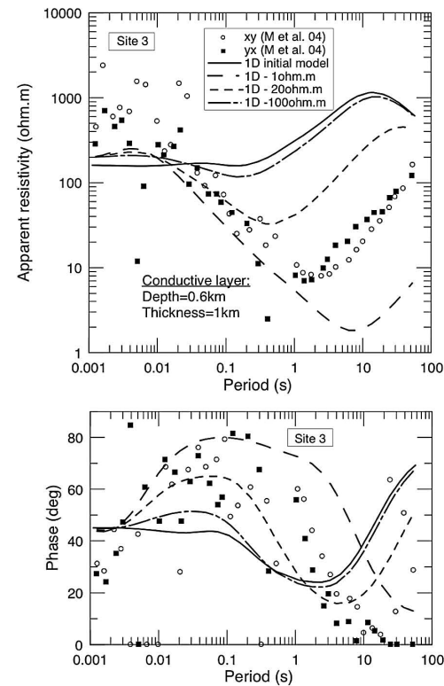
A) Superficial conductor - effect of resistivity
