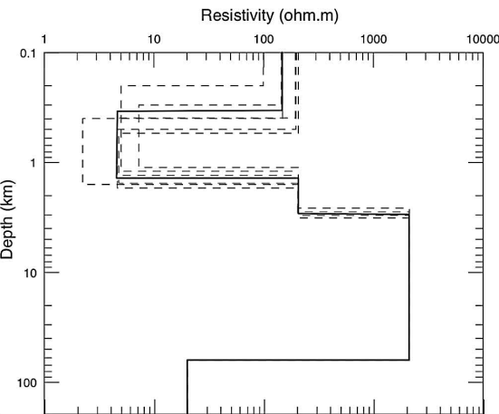
C) Superficial conductor - resistivity profiles vs depth
