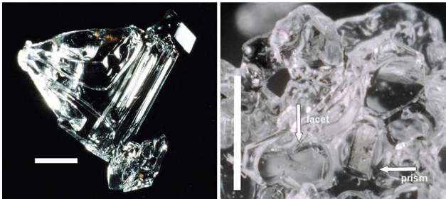
Fig. A2. Left: depth hoar crystal, showing the coexistence of faceted and rounded shapes. Right: melt-freeze crust, showing faceted shapes, even though melt-freeze crusts are often thought to consist only of rounded shapes. Scale bars: 1 mm.
