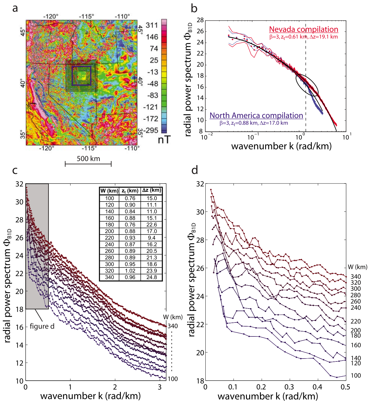
Figure 3. (a) Portion of the aeromagnetic compilation of North America. The black squares indicate the limits of the windows used to compute the radial power spectra presented in Figures 3c and 3d. The bold blue square represents the limits of the window used to compute the radial power spectra presented in Figure 3b. (b) Radial power spectra calculated from Nevada (red) and North America compilations (blue), with a window size of 200 km. The dots and the thin solid colored lines represent the radial power spectrum and the 95% confidence interval \alpha_{95} , respectively. The bold black curves are theoretical curves for a model of fractal random magnetization that best fit the calculated power spectrum, assuming a fractal parameter \beta = 3 . Results of these fits, depth to the top z_t , and thickness of magnetic layer \Delta z , are indicated on the top for the Nevada compilation and on the bottom for the North America compilation. These fits were performed using wave numbers ranging from 0 to 3 rad/km for the Nevada compilation and 0 to 1.4 rad/km for the North America compilation. (c) Radial power spectra calculated for different window sizes, from 100 km (in red) to 340 km (in blue). The table, in the top right corner, shows the results of the fit, performed using wave numbers between 0 and 1.4 rad/km as a function of the size of the window. (d) Expanded portion of Figure 3c represented by the gray square showing the long-wavelength (low wave number) part of the spectra.
