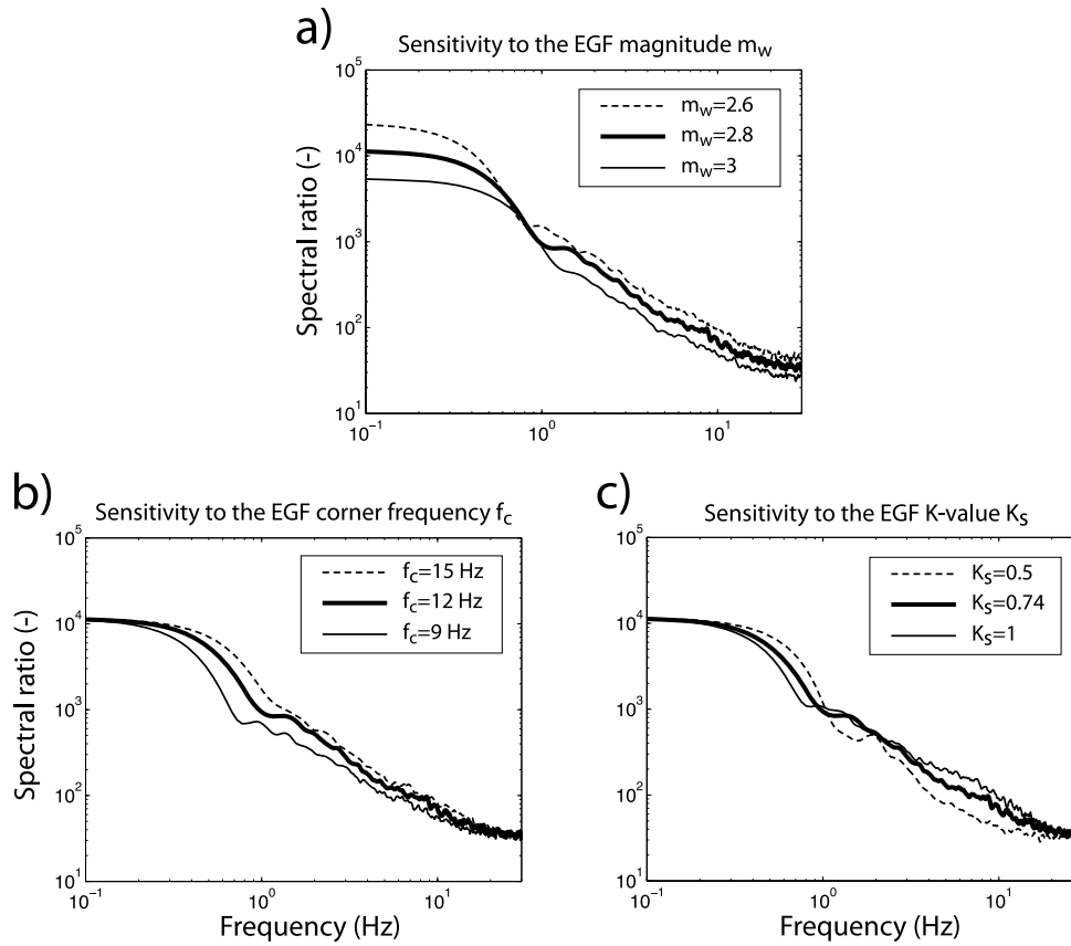
Figure 7. Sensitivity of the ASTF to the EGF parameters M_W , f_c and K_S . The assumed reference values are M_W = 2.8 , f_c = 12 Hz and K_S = 0.74 . The spectra correspond to the quadratic mean of 100 simulated spectra for \Theta = 90^\circ and \tau_{\max} = 0.6 s.
