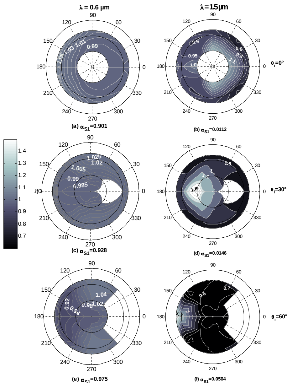
Fig. 5. Ratio of the anisotropy factor R between samples S1 and S3 \left(\frac{R(S1)}{R(S3)}\right) at 0, 30 and 60^\circ incident beam and for two wavelengths. The spectral albedo used to calculate R for S1 is indicated below each chart. S3 spectral albedo is indicated in Fig. 4.
