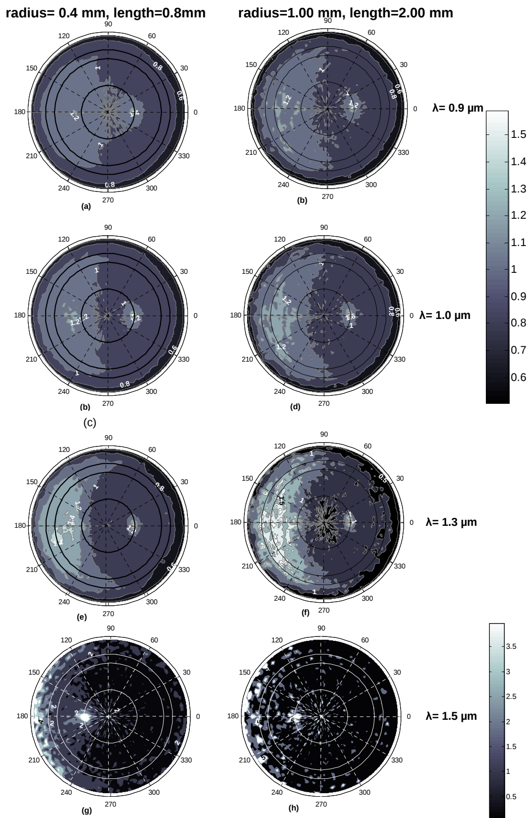
Fig. 9. Anisotropy factor R(\theta_v, \phi) computed with SnowRAT (Picard et al., 2008) for cylinders with random orientation. Incident angle is 30^\circ . Circles at 30^\circ , 60^\circ and 70^\circ viewing angles are drawn on each polar chart.
