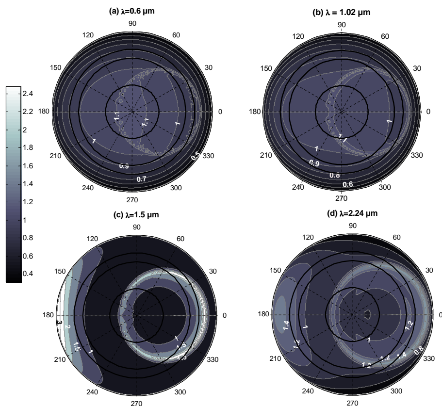
Fig. 8. Anisotropy factor R(\theta_v, \phi) (Mishchenko model, Mishchenko et al., 1999) for spheres with power law distribution of size. Incident angle is 30^\circ . Effective radius is 0.1 \text{ mm} and effective variance of grain size distribution is 0.2 \mu\text{m} . Circles at 30^\circ , 60^\circ and 70^\circ viewing angles are drawn on each polar chart.
