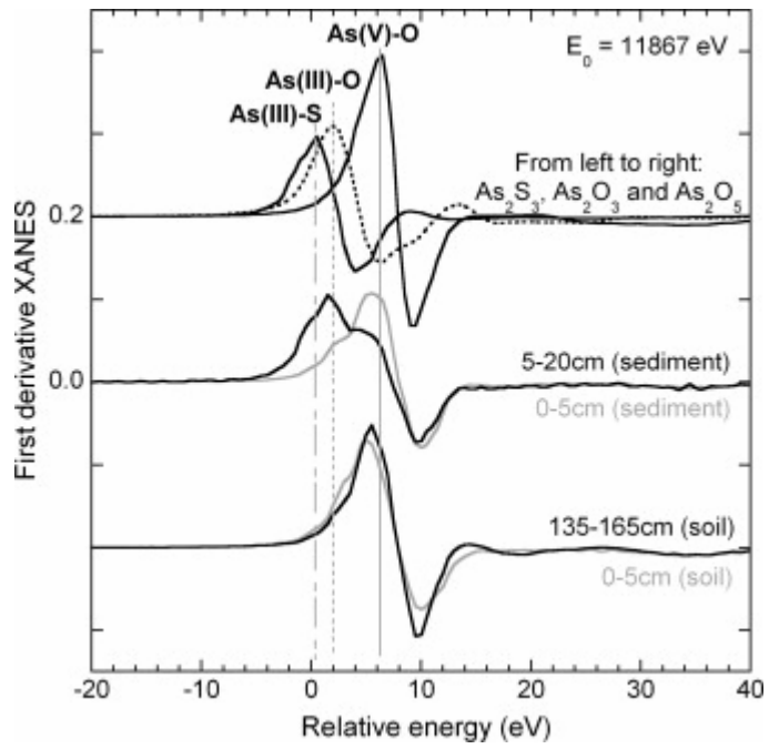
Fig. 3. First derivative As K-edge XANES spectra for the sediment and soil samples compared to reference As compounds of As_2S_3 , As_2O_3 and As_2O_5 as representative species of As(III)-S, As(III)-O and As(V)-O respectively.
