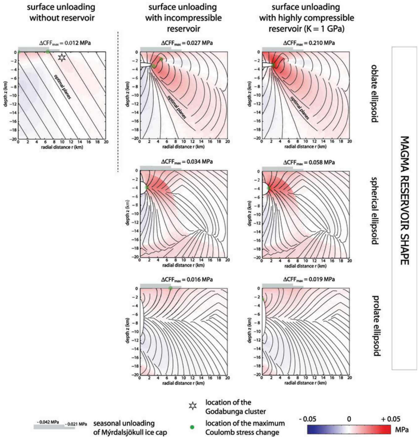
Figure 9. Coulomb stress change ( \Delta CFF ) induced by the seasonal melt of snow at Katla volcano. \Delta CFF is calculated on planes optimum for shear failure (shown with black lines) when the magma chamber is pressurized, with a surrounding lithostatic stress field. Parameters of the seasonal unloading as well as the chamber geometry are described in Table 3. Values of Young’s modulus, Poisson’s ratio and effective internal friction coefficient used are, respectively, 30 GPa, 0.25 and 0.5. Various reservoir shape (ellipticity equal to 5, 1 and 1/5) and magma compressibility are considered. In the top left panel, Coulomb stress change for a ‘reference case’ without magma chamber is calculated for an extensive regime associated with normal faulting. An indication of the location of the Godabunga cluster is shown (black star). For each model, location (green dots) and amplitude value of the maximum of Coulomb stress change is detailed.
