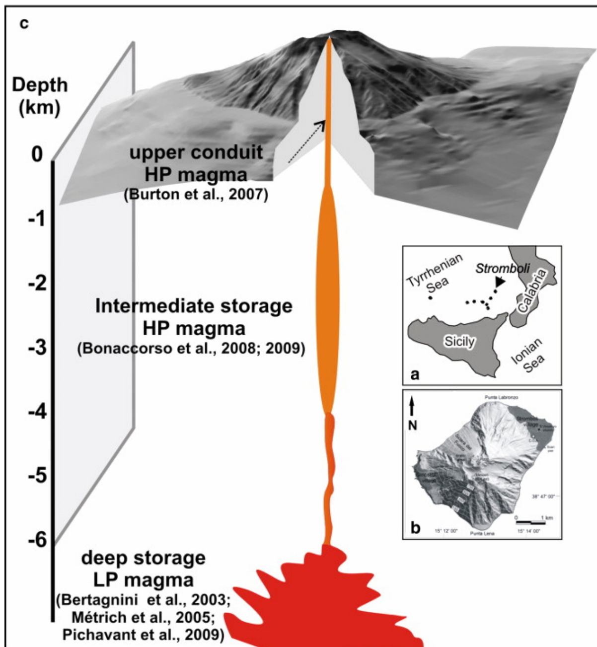
Fig. 1. : (a) Aeolian Islands and position of Stromboli in the southern Tyrrhenian Sea. (b) Map of Stromboli island. (c) Simplified section of Stromboli feeding system, showing the upper conduit extending from the magma surface (750 m a.s.l. corresponding to the elevation of the summit craters) to ~ 2 km b.s.l. (Burton et al., 2007), and the intermediate storage system (2–4 km depth; [Bonaccorso et al., 2008] and [Bonaccorso et al., 2009]). These both contain HP magma, whereas the deep magma storage zone, below 6 km depth, contains LP magma (e.g., [Bertagnini et al., 2003], [Métrich et al., 2005] and [Pichavant et al., 2009]).
