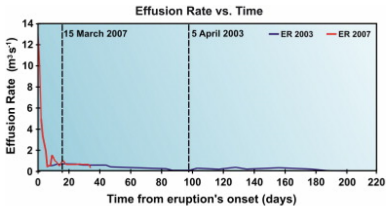
Fig. 3. Comparison of the effusion rates ( \text{m}^3 \text{s}^{-1} ) measured during the 2002–2003 ([Calvari et al., 2005a], [Calvari et al., 2005b] and [Lodato et al., 2007]) and the 2007 (Calvari et al., 2010) eruptions vs. time (days) from eruption's onset. Note that for both eruptions effusion rate values are here reported as 7-day-moving averages.
