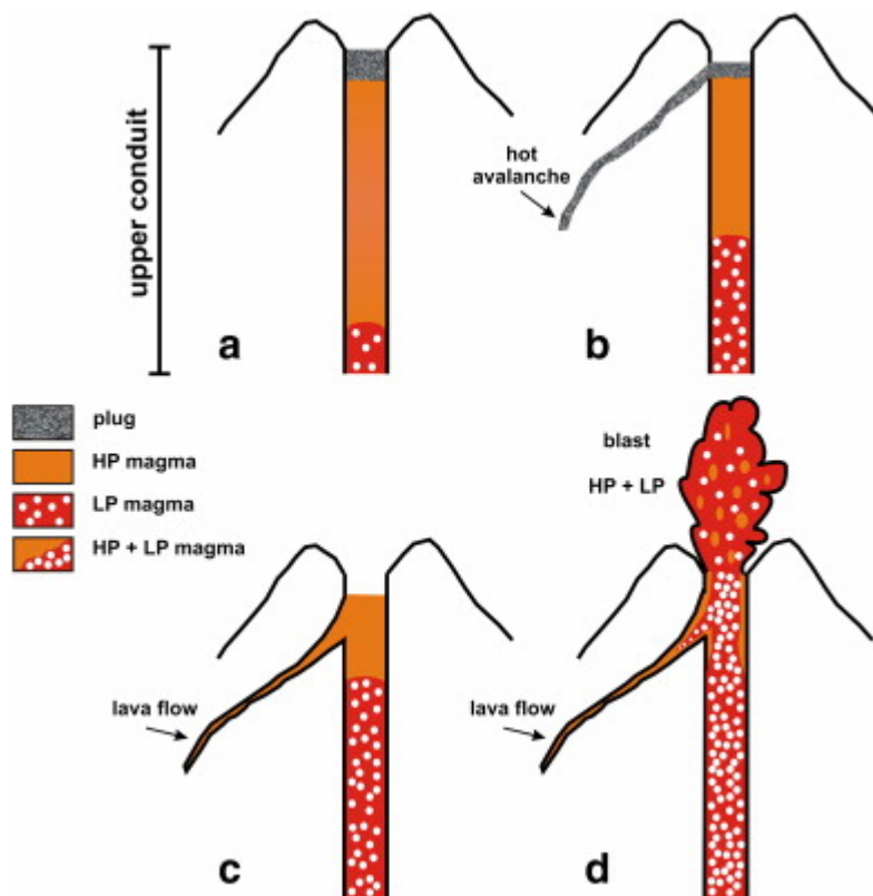
Fig. 5. Sketch showing the upper conduit of Stromboli, with phases of less-porphyrific (LP) magma rising, and its relationships with the high-porphyricity (HP) magma. (a) The upper conduit before the onset of an effusive eruption. (b) The plug removed during the initial phases of an effusive eruption (crater breaching and hot avalanche spreading). (c) Effusive vent opening and lava flow draining the upper, HP magma column. (d) LP magma erupting explosively (paroxysm) and being drained through the effusive vent, mixing with the HP magma.
