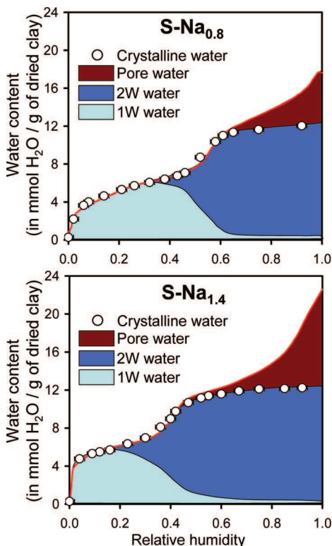
Figure 8. Relative contributions of the different types of \text{H}_2\text{O} molecules along the water vapor desorption isotherm. The total water content determined from gravimetric experiments is corrected for the presence of residual water (see text for details). The contribution of water in meso- and/or macropores is calculated as the difference between the total water content and the contribution of crystalline water present in 1W and 2W interlayers.
