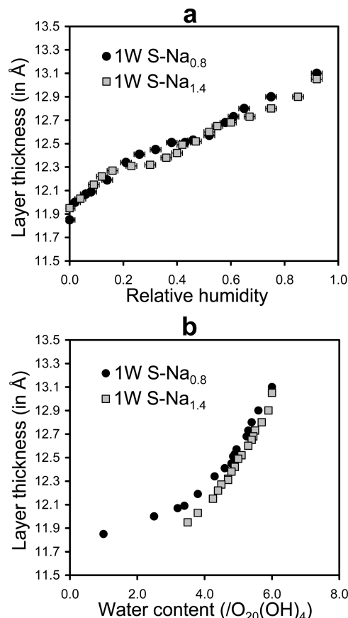
Figure 4. Evolution of monohydrated layer thickness as a function of (a) relative humidity and (b) interlayer water content. Solid circles and gray squares represent results obtained for S-Na 0.8 and S-Na 1.4 , respectively.
