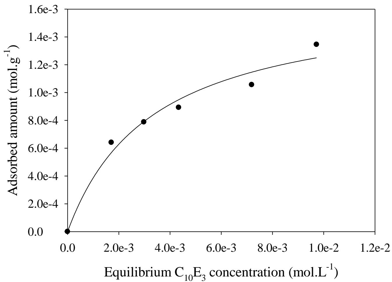
Figure 2: Intercalation of a Nonionic Surfactant ( C_{10}E_3 ) bilayer into a Na-Montmorillonite Clay
