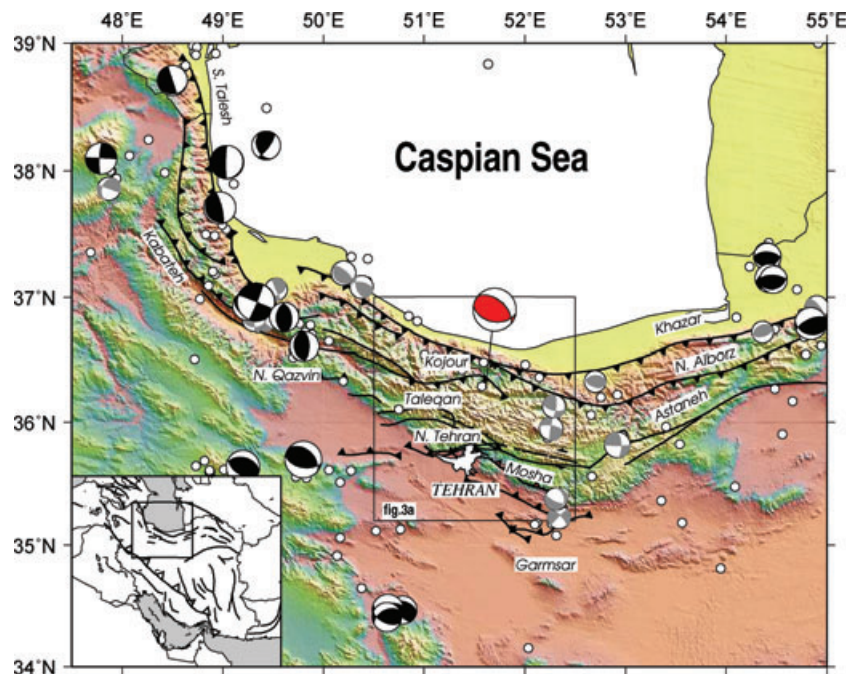
Figure 1. Topography, earthquake locations and focal mechanisms across the Alborz Mountains. Black focal spheres are for earthquakes where the mechanisms are constrained by body waveform modelling (Priestley et al. 1994; Jackson et al. 2002); grey focal spheres are Harvard CMT solutions for events with M_w \geq 5.3 and with \geq 70 per cent double-couple component. The red focal spheres is the 2004 Baladeh earthquake whose focal mechanism was also determined by waveform modelling (Tatar et al. 2007). Size of the focal spheres are proportional to magnitude. White circles are seismicity from Engdahl et al. (2006). The known major faults in the region are indicated. The inset map at lower left shows the location of the central Alborz Mountains with respect to the more broad-scale features of the Arabian–Eurasian collision zone. The box denotes the location of the temporary seismic network in the central Alborz Mountains.
