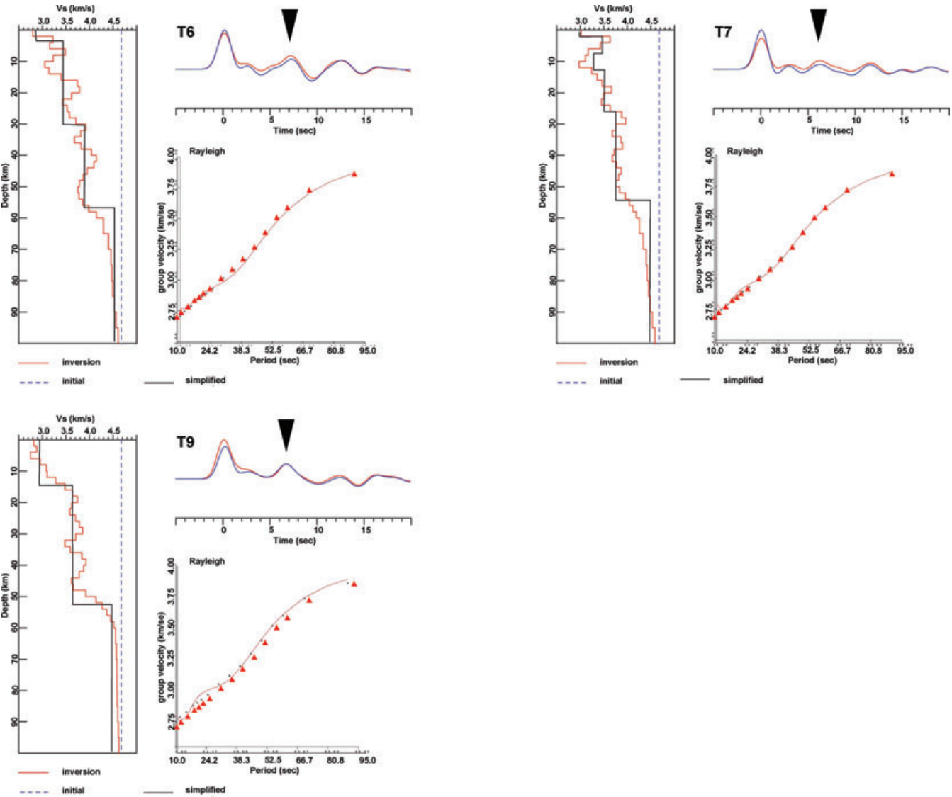
Figure A4. Receiver function and surface wave analysis for the sites T6, T7 and T9. The number of receiver function stacks inverted and the total number of receiver function included in the receiver function stacks is given in Table 1. The format of the figure is the same as that in Fig. 2.
