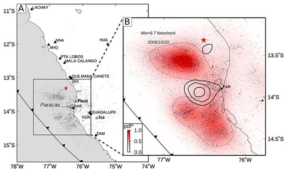
Figure 11. (a) Distribution of aftershocks recorded by a local IGP seismological network (triangles) during the 45 days following the main shock. (b) Zoom on the area of large aftershock activity. A normalized probability density function for this catalog is shown in red color, with thin red contours every 0.3 of a unit. Also indicated are 2 m contours of slip 2 m from the joint inversion (black contours). The red star is the epicenter of the 2007 Pisco main shock, and the yellow star shows the location of the large M_w 6.7 foreshock of 20 October 2006.
