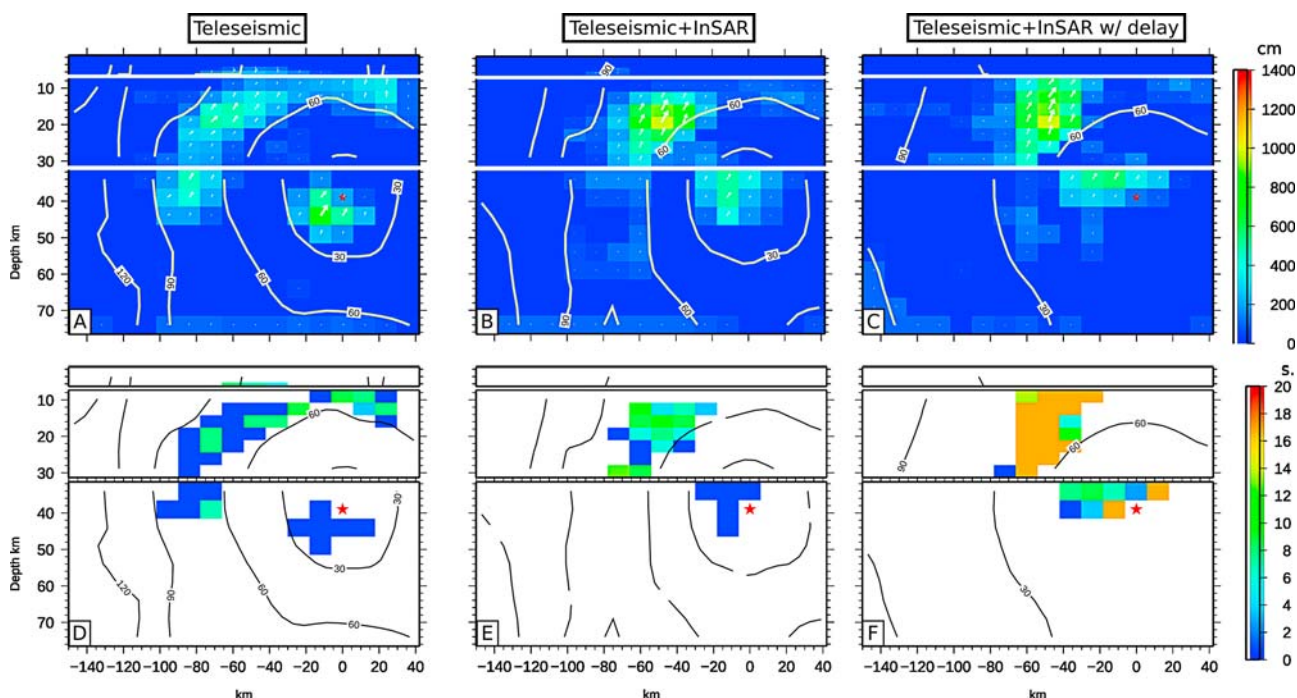
Figure 10. Head-on view of the (a–c) slip and (d–f) risetime distributions on the fault segments obtained from the teleseismic (Figures 10a and 10d), joint inversion of teleseismic and InSAR data using a low rupture velocity (0.8–1.2 km/s; Figures 10b and 10e), or faster rupture velocity (2.4–2.8 km/s) with an imposed 38 s time delay of the rupture front between the two lower segments (Figures 10c and 10f). Color levels correspond to the amount of slip or duration of the risetime on a given subfault, with the direction of slip indicated by the white arrows. On the right hand side, the risetime value is only shown for subfaults that experience more than 200 cm of slip.
