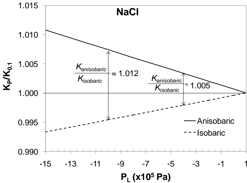
Figure 5. K_P/K^\circ ratio for NaCl precipitation as a function of capillary pressure, according to the isobaric and anisobaric contexts (see text; thermodynamic properties from the Thermoddem database, available at http://thermoddem.brgm.fr/ ).
