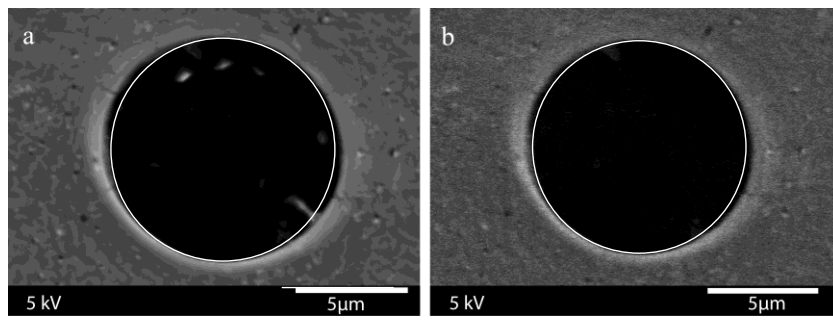
Figure 3. Two pores of the 10 µm membrane of figure 2, once the precipitated salts were removed by dilution. The membrane keeps deformed and seems micro-cracked, demonstrating the potential geomechanical power of the in-pore capillary traction.
