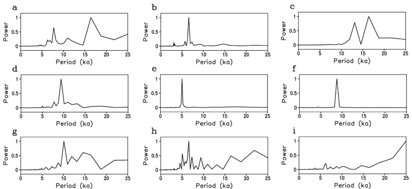
Fig. 3. Power spectrum of the average ice thickness over the sediment area in run ST (see Fig. 2) for each model in the intercomparison. The maximum power has been normalized to unity for each model separately.
