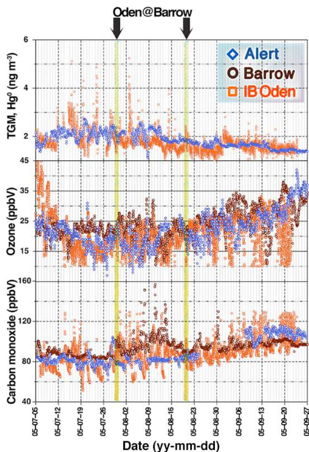
Fig. 6. Comparison of Oden (orange squares), Barrow (brown circles) and Alert (blue diamonds) observations for TGM, \text{Hg}^0 (upper panel), \text{O}_3 (middle panel) and for CO (lower panel). The time series from IB Oden depicted are comprised of 10-min averaged data while the others refer to hourly averaged data. Periods shaded in yellow resemble anchorage time of IB Oden outside Pt. Barrow.
