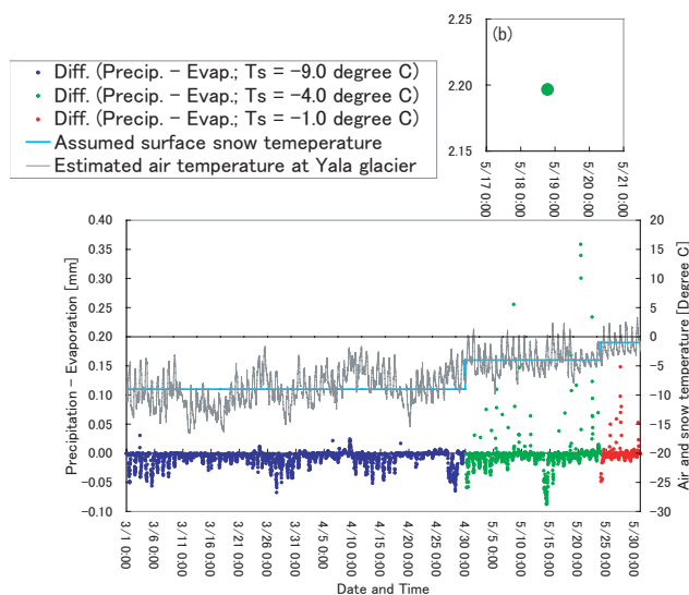
Fig. 5. Difference between precipitation ( P ) and estimated evaporation ( E ) (sublimation in this study). The constant snow surface temperatures of -9 , -4 , and -1 ° were used during 1 March–29 April, 30 April–23 May, and 24 May–31 May, respectively. One data in P - E at the time of Event A was located out of range and plotted in Fig. 5b separately. In Fig. 5b, vertical and horizontal axes have the same units as Fig. 5a.
