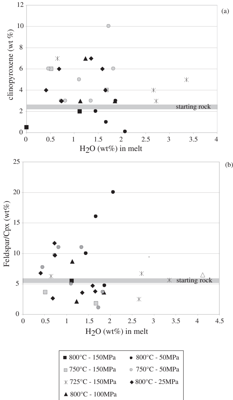
Fig. 3. (a) Variation of clinopyroxene proportions (wt %) in experimental charges with melt water content ( H_2O_{melt} ); (b) variation of Feldp/Cpx weight ratio in experimental charges. In both panels the grey bands correspond to the parameter value in the starting rock.
