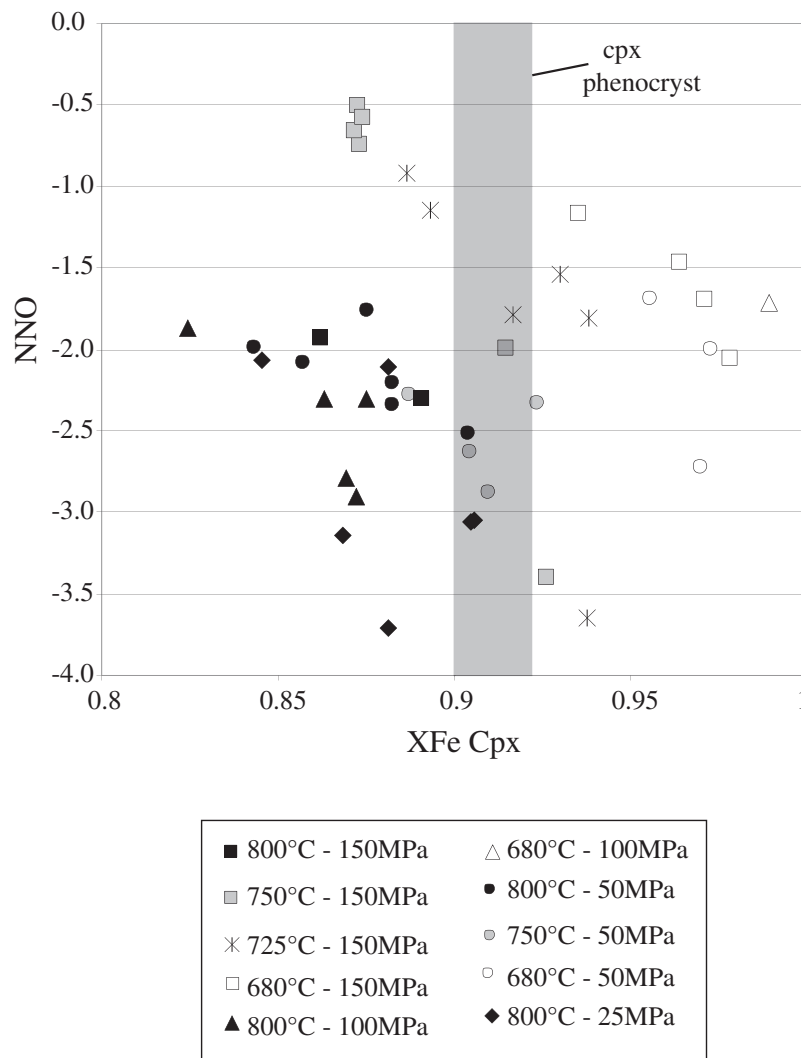
Fig. 7. Variation of X_{\text{Fe}_{\text{tot}}} [\text{Fe}_{\text{tot}}/(\text{Fe}_{\text{tot}} + \text{Mg})] of experimental clinopyroxenes with oxygen fugacity expressed as \Delta\text{NNO} at a range of temperatures and pressures. The grey band corresponds to the average X_{\text{Fe}} value of clinopyroxene phenocrysts in the starting rock.
