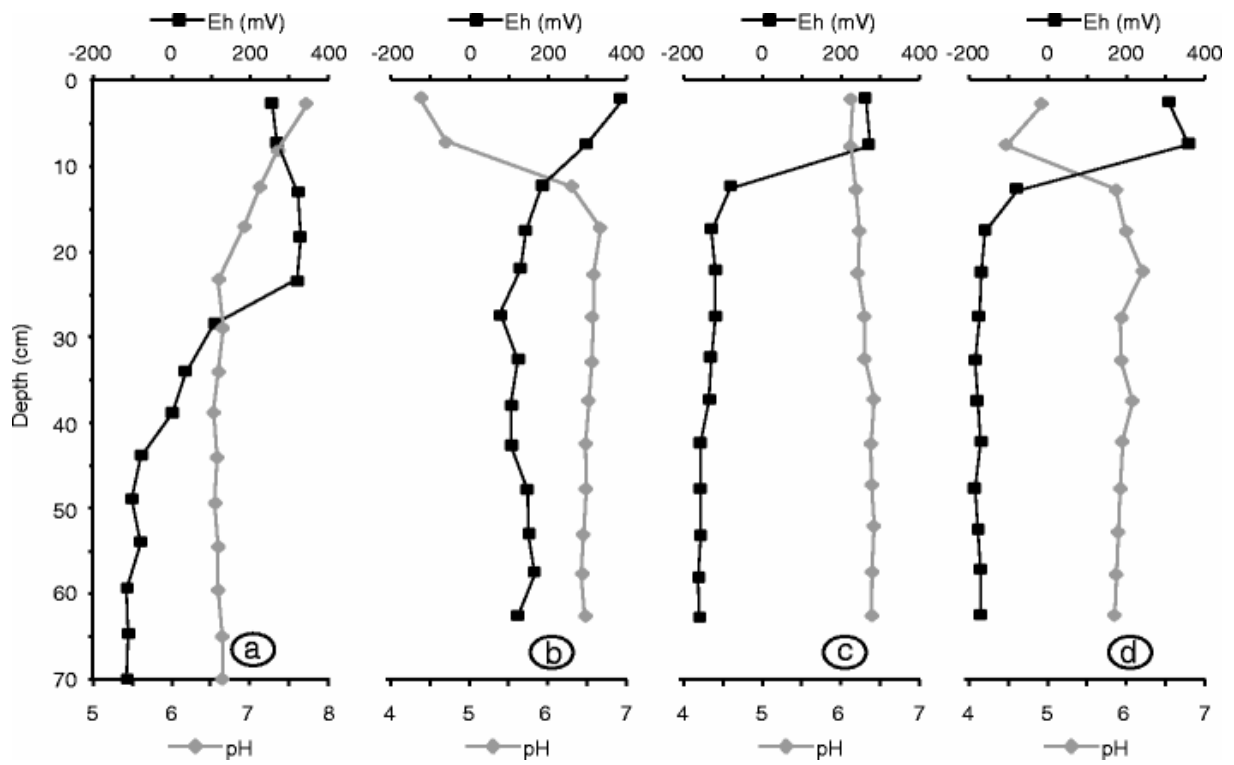
Fig. 3 Depth distribution of redox and pH without effluent in the various sites: a) salt-flat; b) Avicennia marina forest; c) dead Rhizophora stylosa forest; d) Rhizophora stylosa forest
