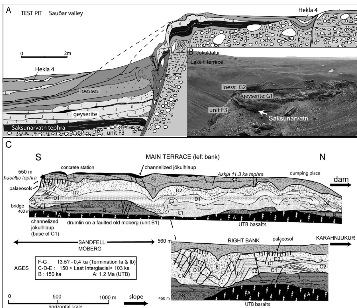
Fig. 5. Deformation structures. A - Early Holocene tectonics (Sauðar valley); B - Glaciotectonic deformations in the Saksunarvatn tephra in the Jökuldalur close to the entrance of Sauðar valley; C - Field sketch of the valley sediments between the bridge (South) and the dam (North). Notice the drumlin form of unit B, in the southern part, and the giant glaciotectonics between the Sandfell and the Kárahnjúkur, within the right bank.
